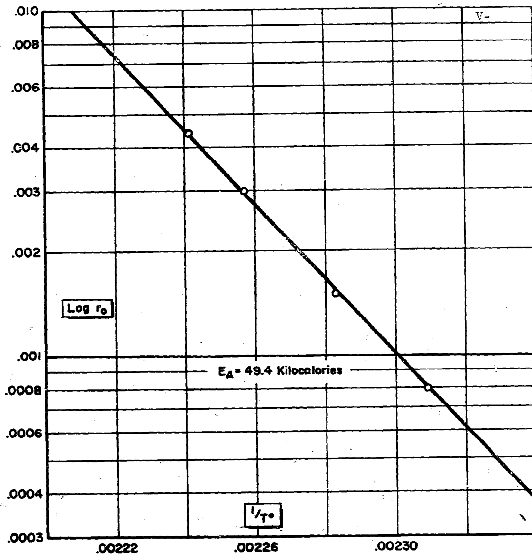
(U) Fig. 26 - Arrhenius Plot; \text{N}_2(+\text{CO}) Rate at Zero Time; Millimoles Gas per Minute per 200 Mg. Poly FA-BDE
