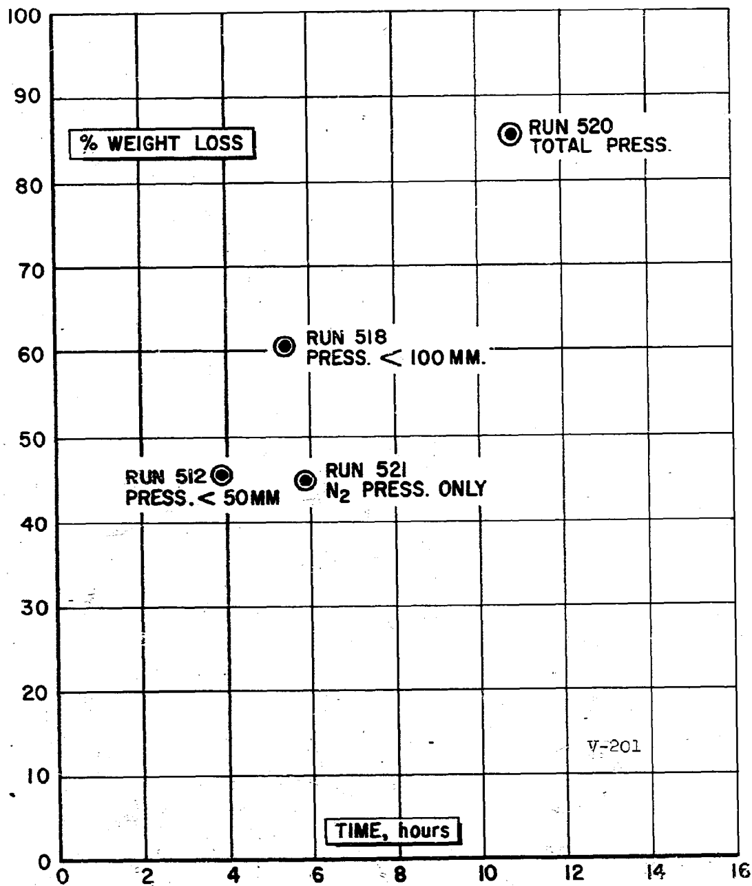
(U) Fig. 2 - Percent Weight Loss of Solid INPO-635P at 170°C. In Monel Reactor.
