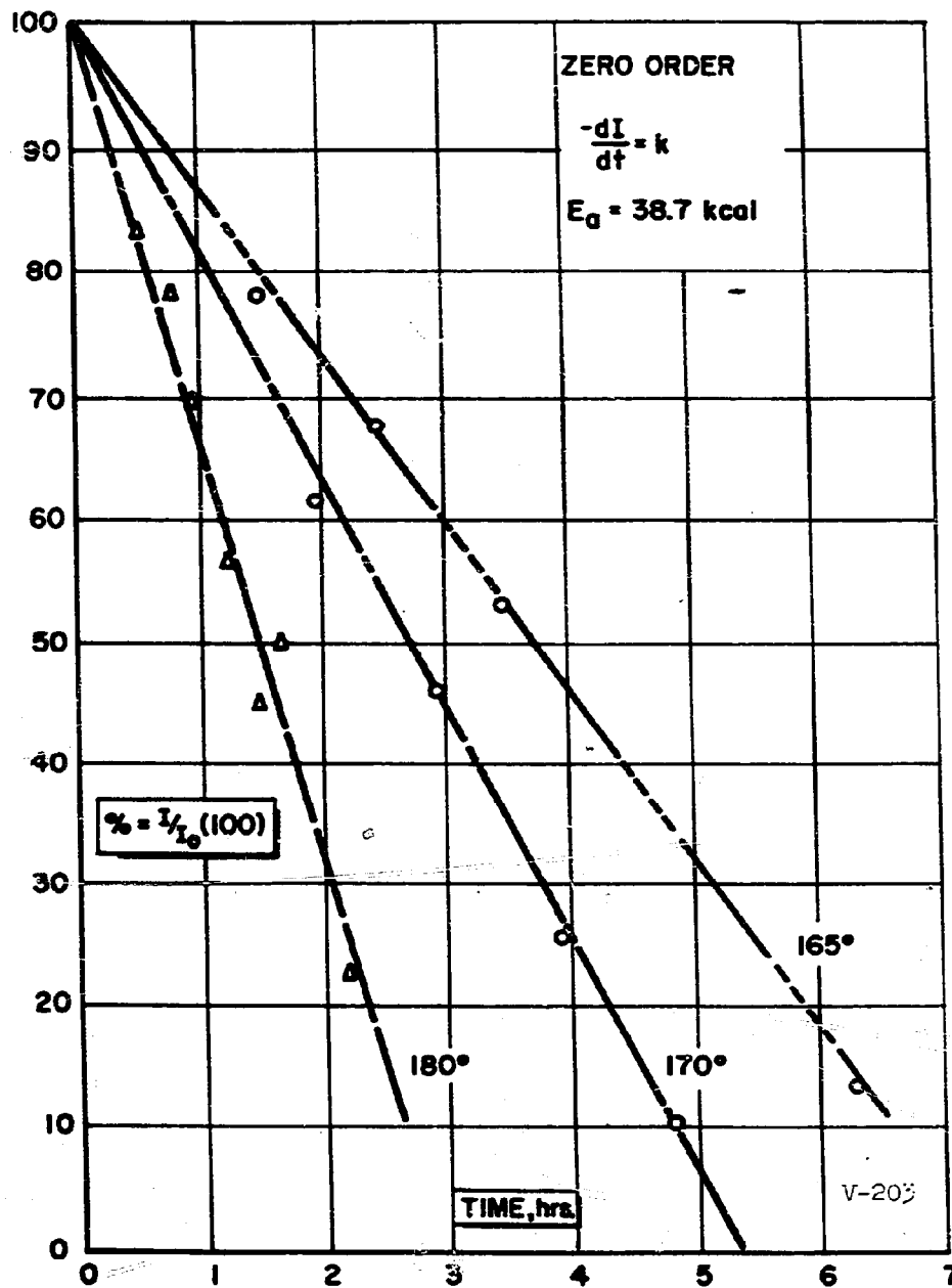
(U) Fig. 7 - Percent INFO-635P Present in Residue
