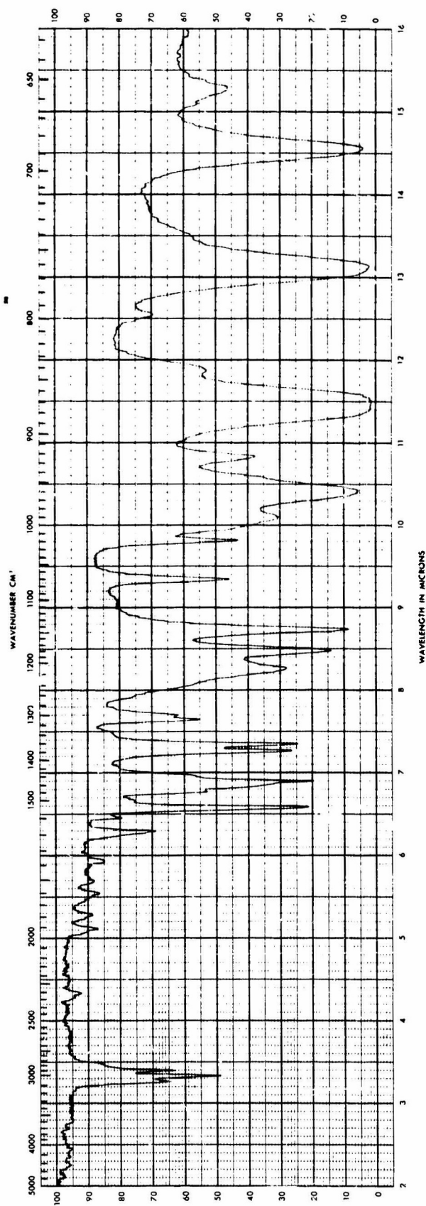
Infrared Spectrum of 2-Phenylazo-2-difluoramino-2-propane
