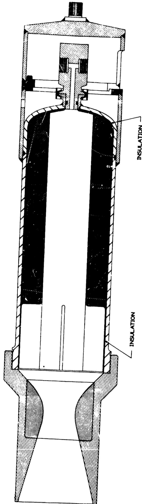
FIG. 1 APPLICATION MOTOR WITH SLOTTED-TUBE GRAIN.
