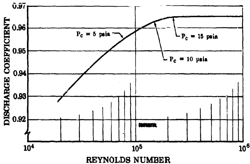
Figure 53. Variation of 8.5K Nozzle Discharge Coefficient
