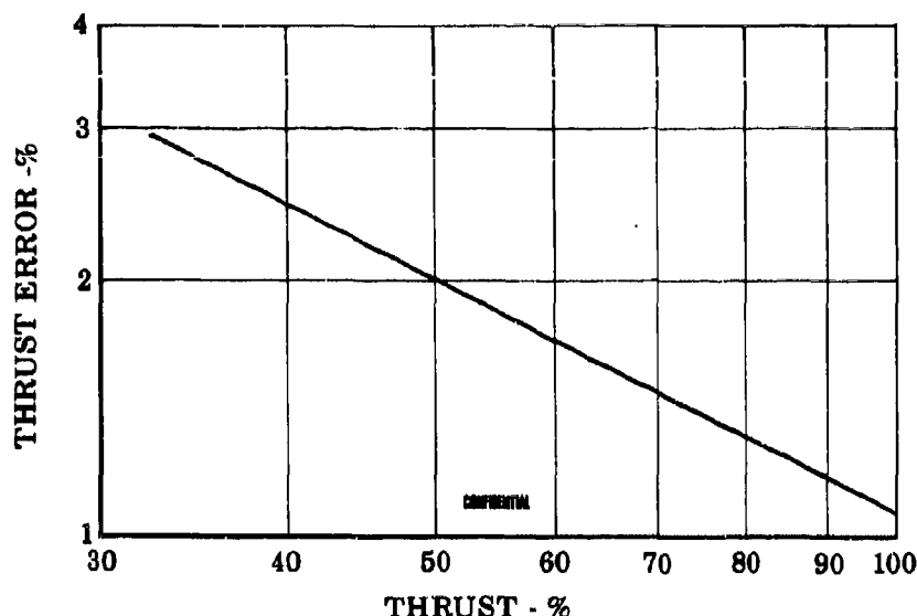
Figure 111. Thrust Error
