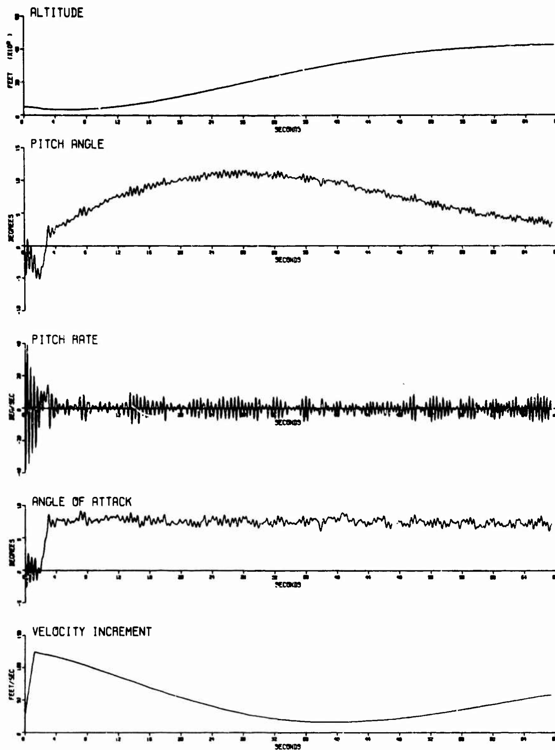
Figure 7.3a RUN 2, TIME HISTORY OF PARAMETERS
