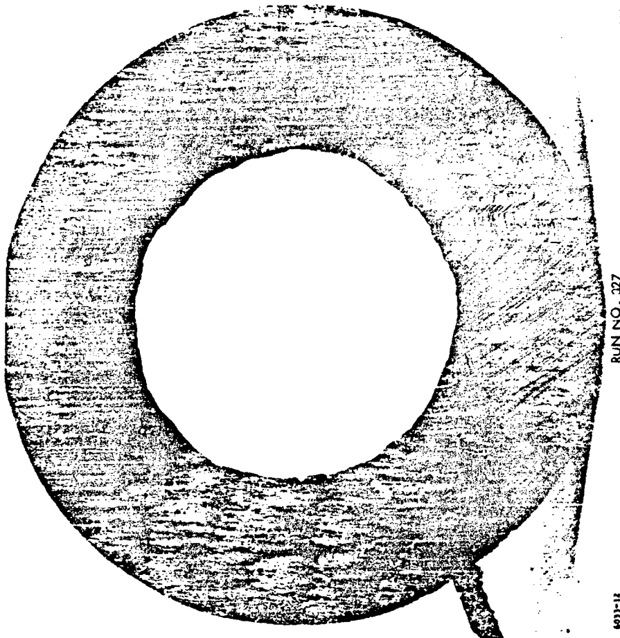
Figure 33. (U) Throat Contour Orientation Insert No. 7
