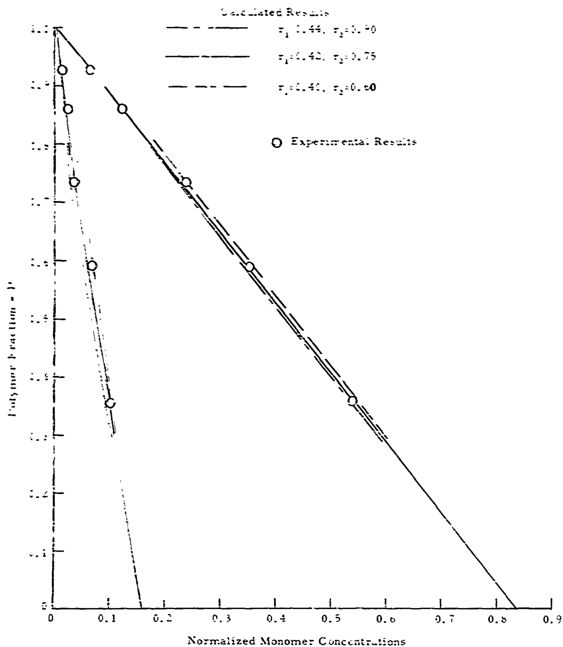
Fig. 7 Normalized Concentration-Conversion Plot, 94/6 NFPA/AA Weight-Ratio Copolymer
