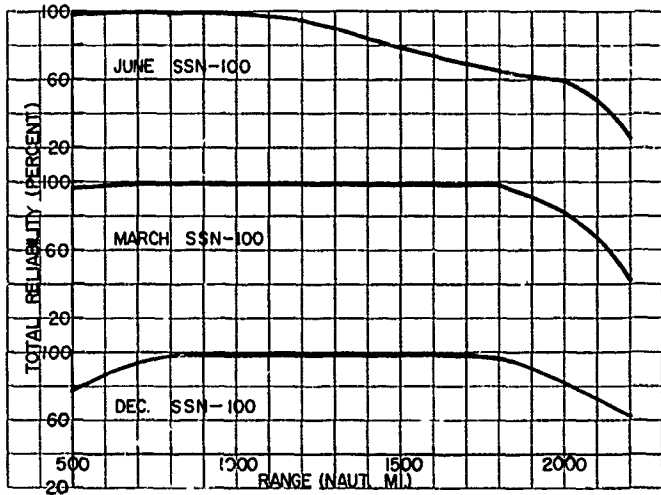
Fig. 15 - Total Reliability averaged over a day, given as a function of range for the three seasons and SSN = 100
