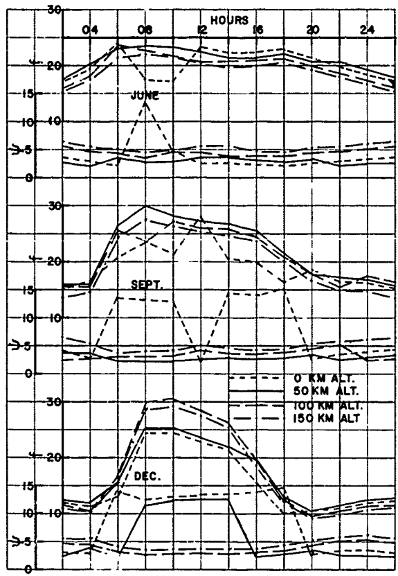
Fig. D4 - The median MUF and its launch angle, shown as combined plots for the altitudes considered
