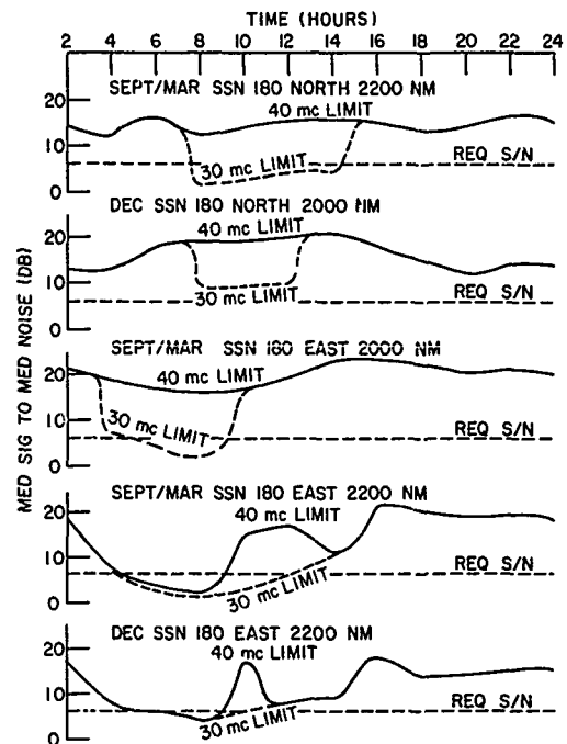
Fig. 9 - Diurnal plots of signal-to-noise ratio for a 30-Mc and a 40-Mc upper limit. At the indicated long ranges, seasons, directions, and SSN = 180, the cases are treated where significant performance improvement is afforded by the 40-Mc upper frequency bound.
