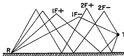
Fig. D1 - The transmission modes considered for targets at altitudes greater than zero sketched for F-layer reflection
