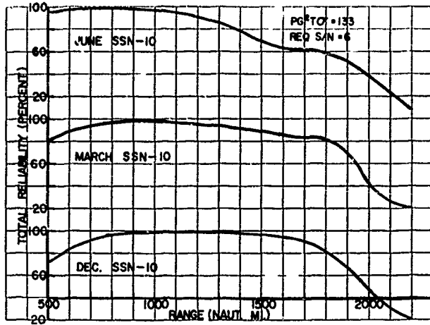
Fig. 13 - Total Reliability averaged over a day, given as a function of range for the three seasons and SSN = 10
