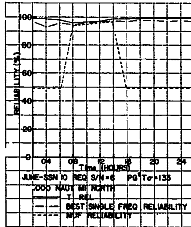
Fig. 4 - The reliability of the median MUF, the reliability of the best single frequency of the complement, and the Total Reliability are given for a 1000-naut-mi case. The E layer is seen to provide the median MUF path between 0800 and 1300 hours.
