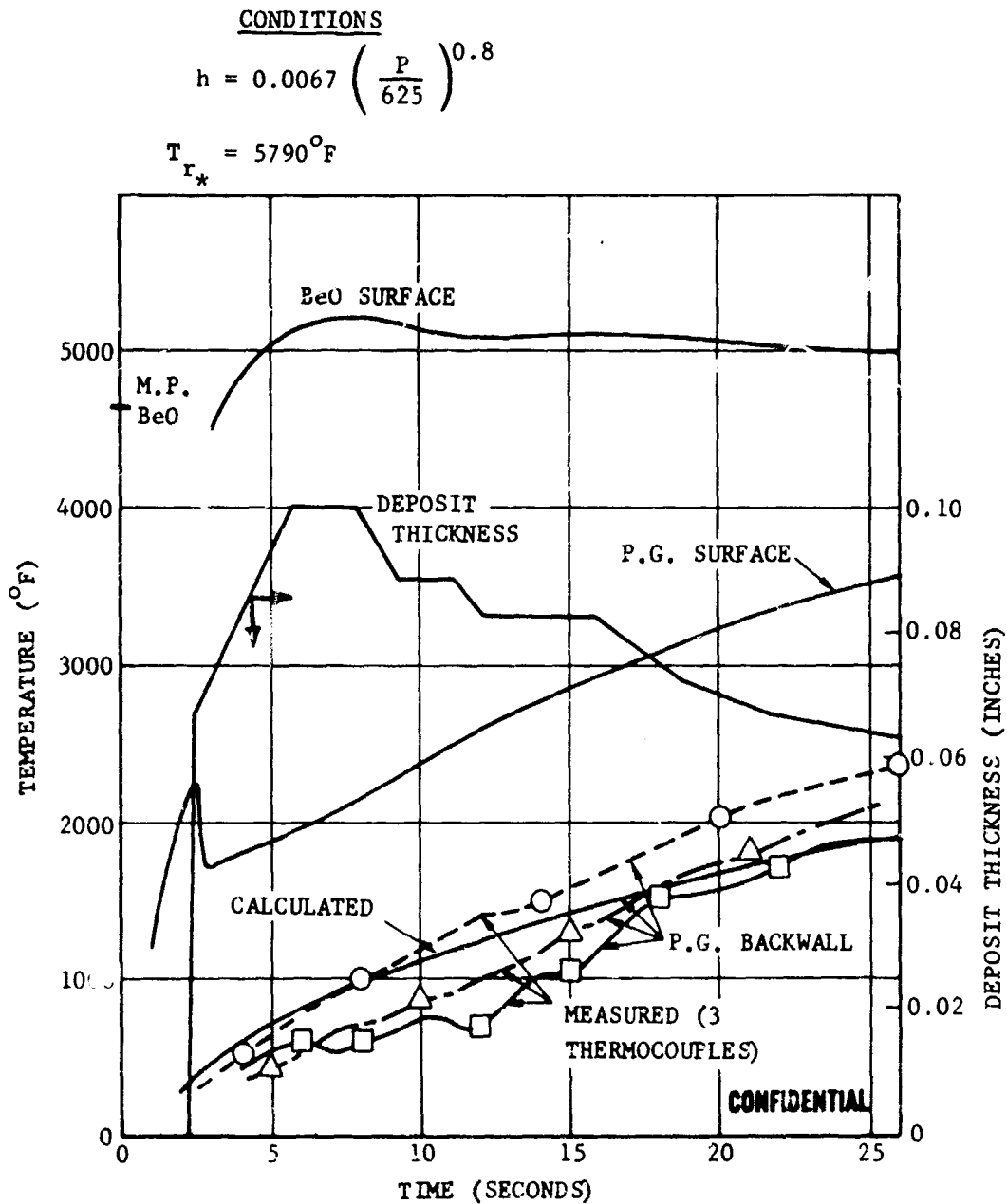
FIGURE 226. THROAT TEMPERATURE RESPONSE WITH DEPOSITION, TEST T-52
