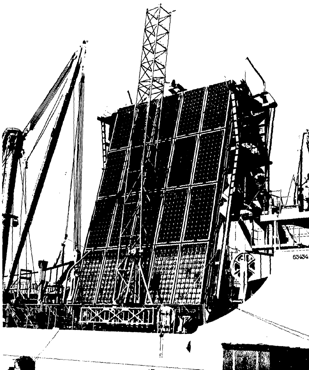
Fig. 4 - Three boom sections attached to array
