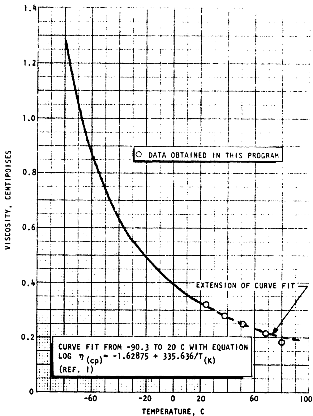
Figure 4. Viscosity of Saturated Liquid Chlorine Pentafluoride
