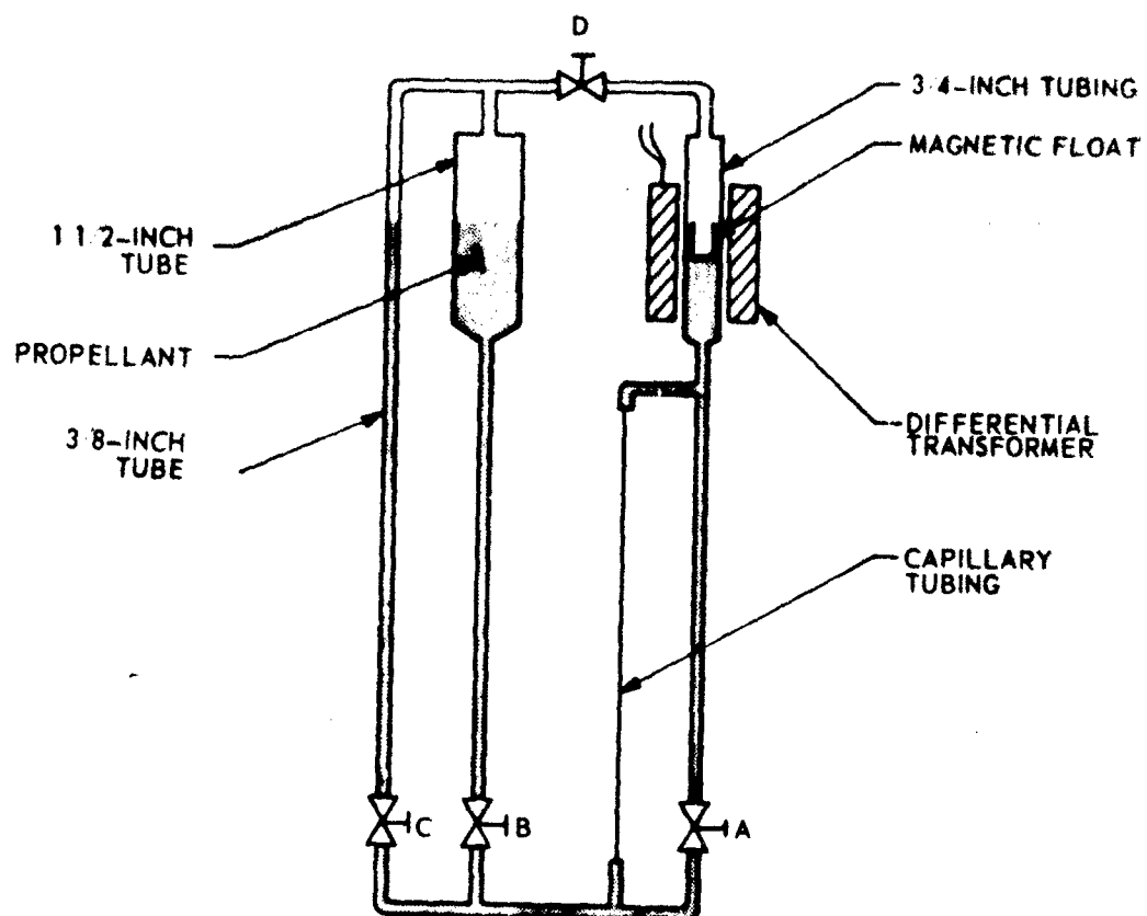
Figure 3. Capillary Viscometer Schematic
