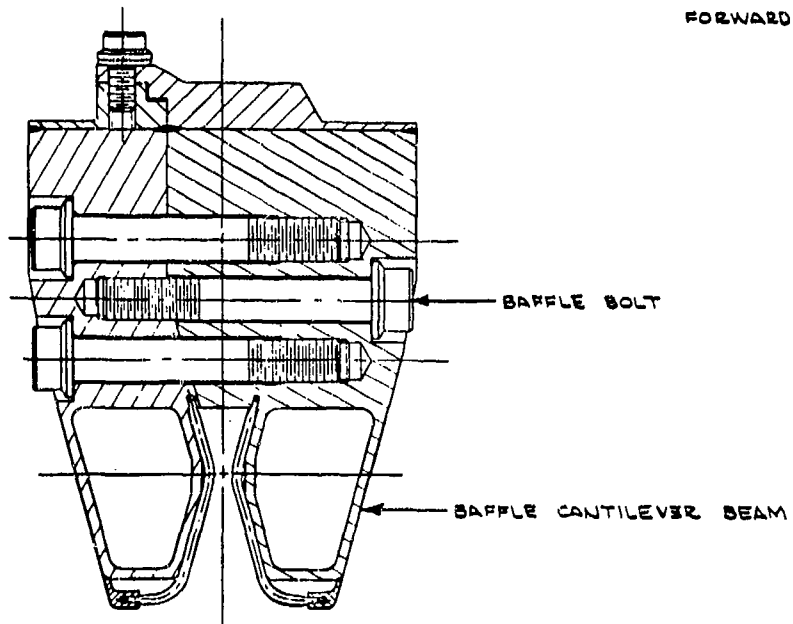
SECTION 13-13
