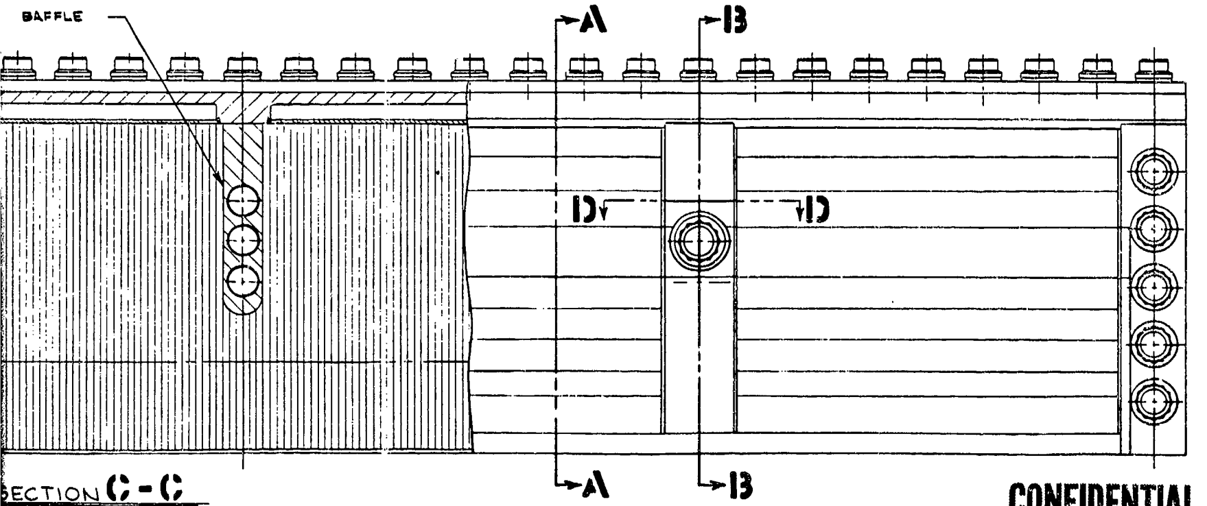
Figure 11 Structural Test Segment - Rib Supports 19/20
