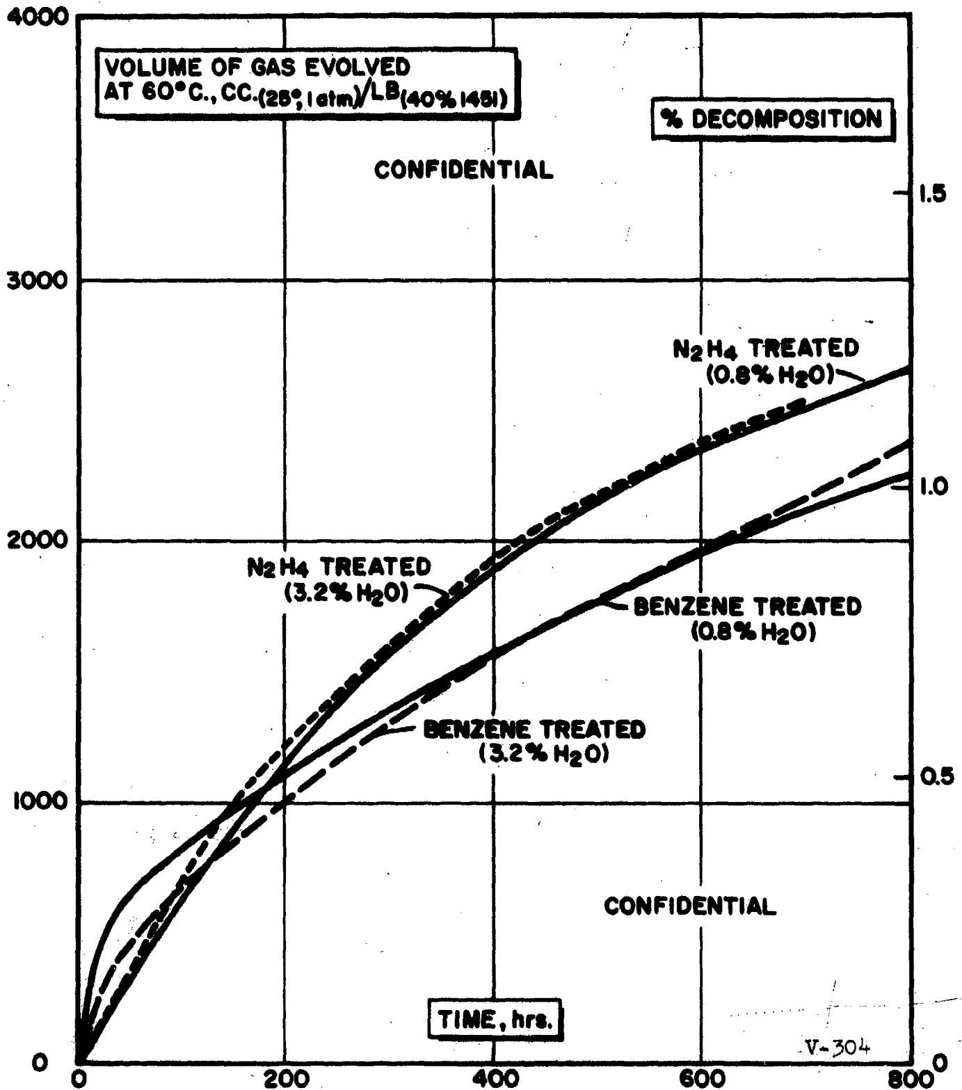
(C) Fig. 7 - Gas Generation of Pretreated Aluminum Hydride-1451 (Lot 09236) in As-Received Hydrazine.
