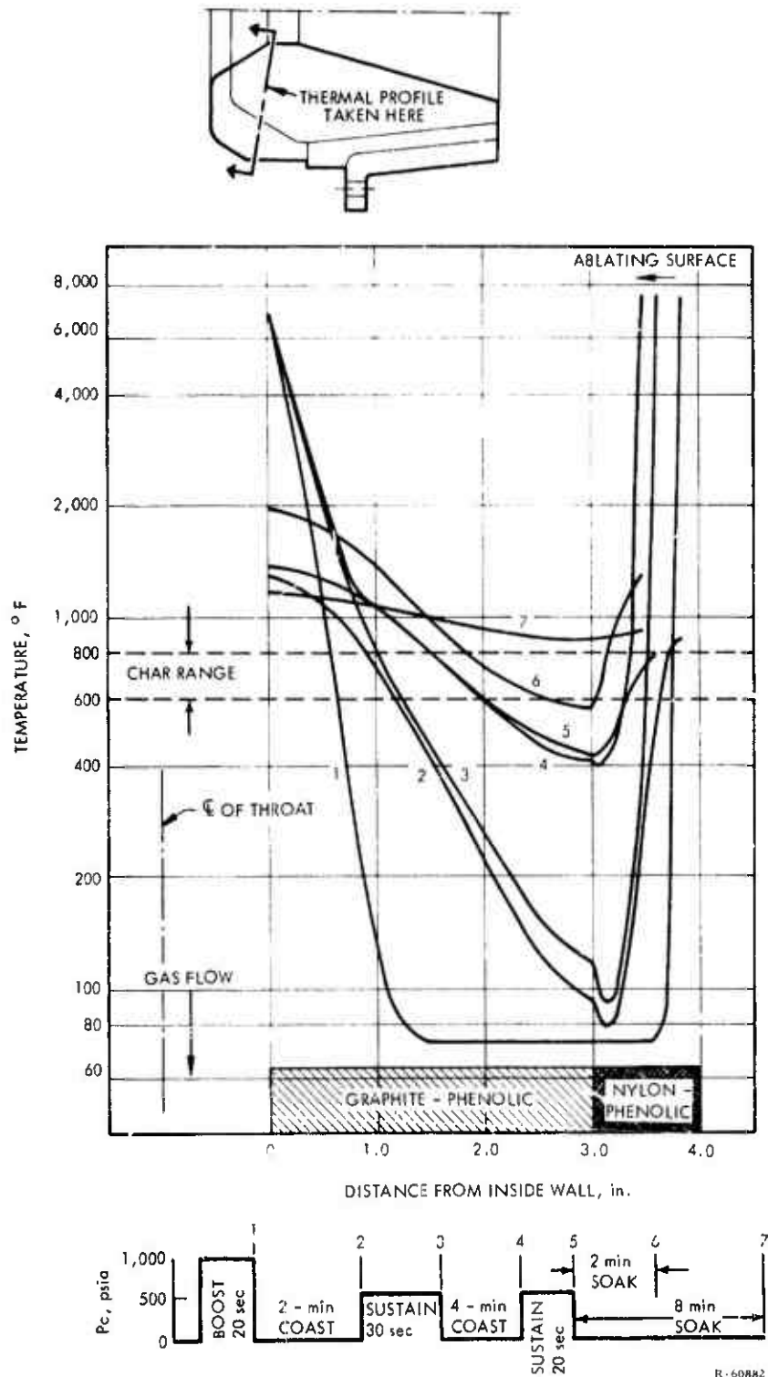
Figure 11. (U) Thermal Profile of Nozzle Throat
