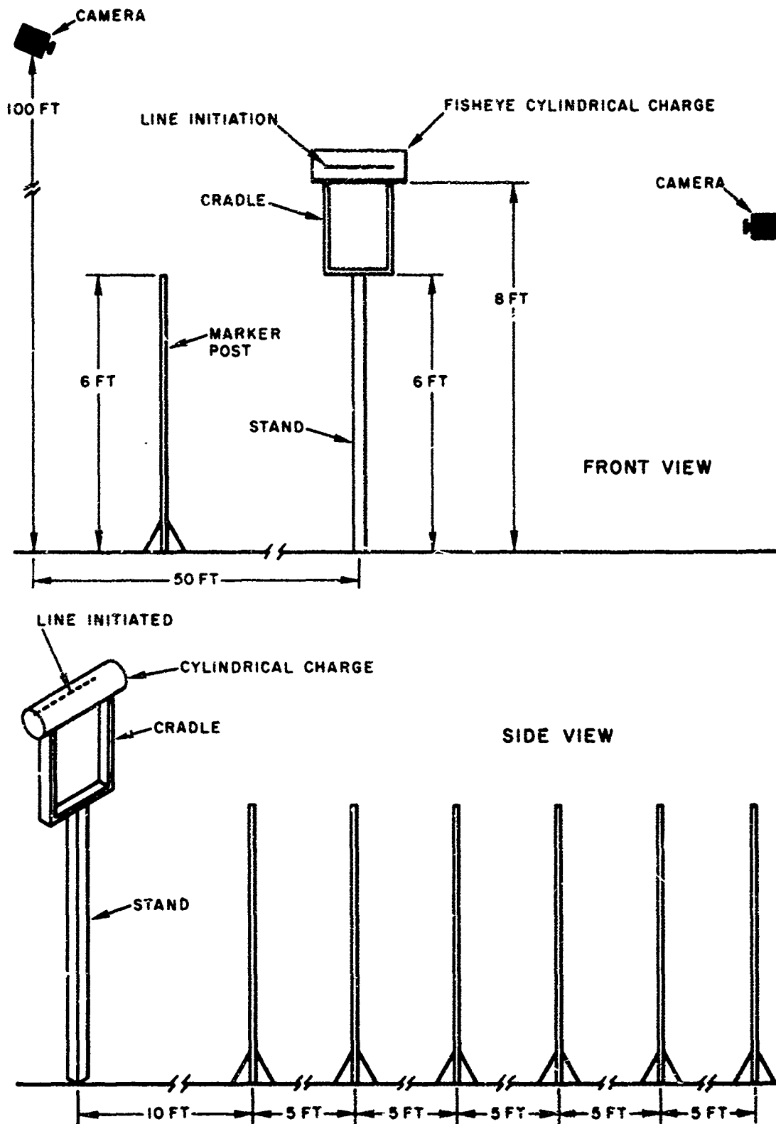
FIGURE 6. Setup for Testing Cylindrical Charges at Chino Arena
