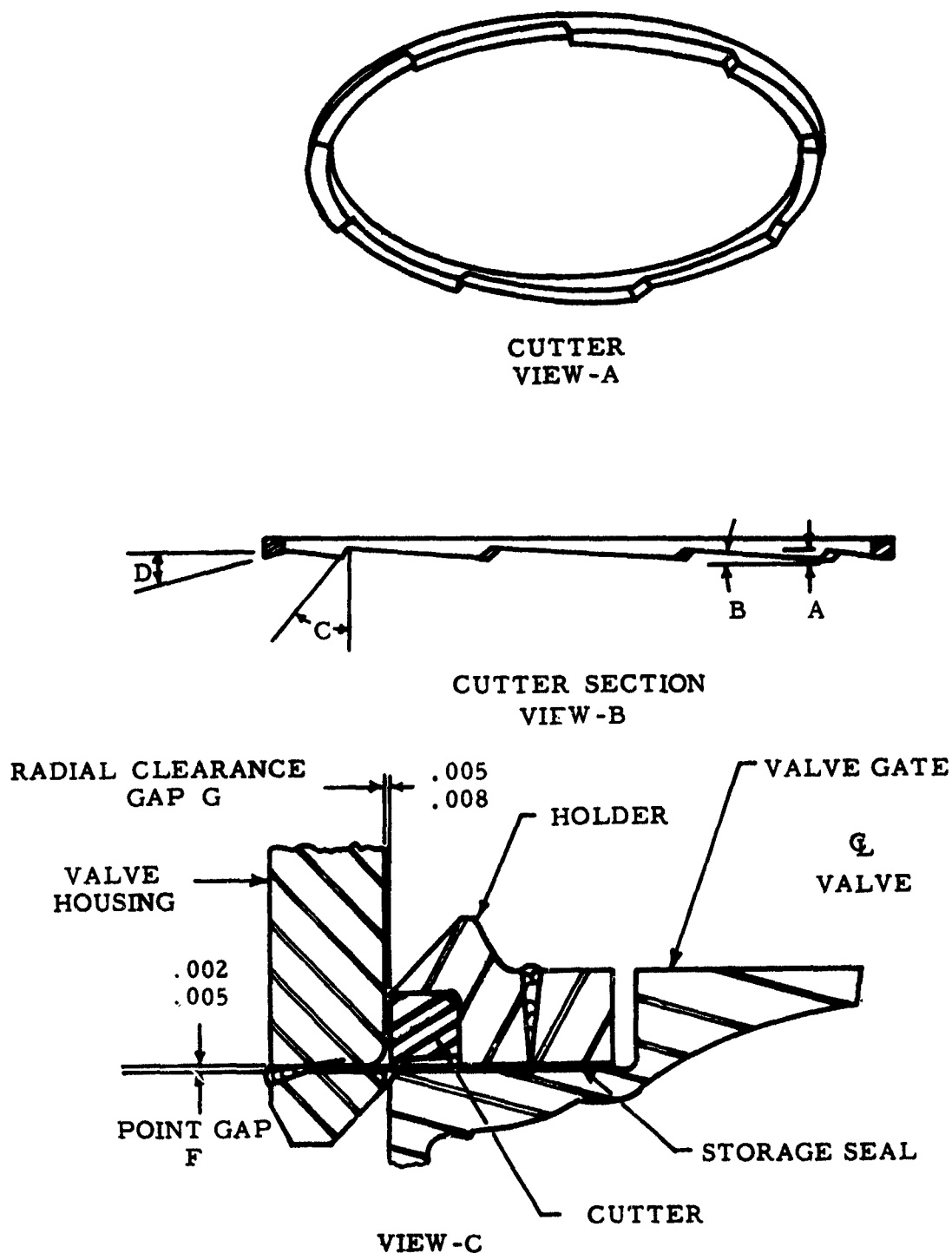
Cutter and Storage Seal Configuration
