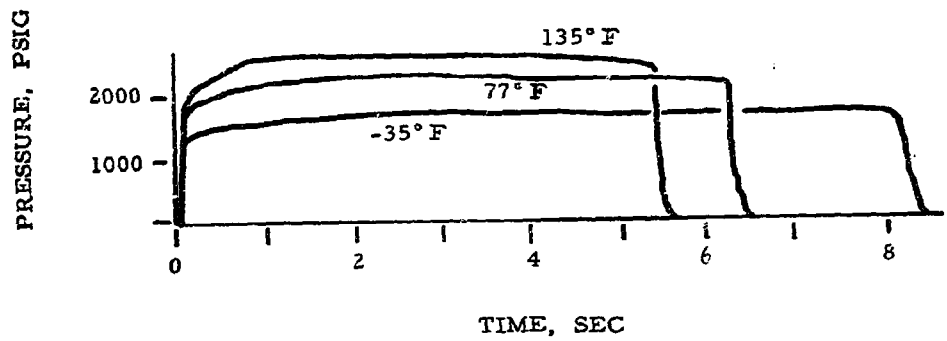
FIGURE 11. (U) PERFORMANCE OF NF REDEYE SUSTAINER MOTORS
