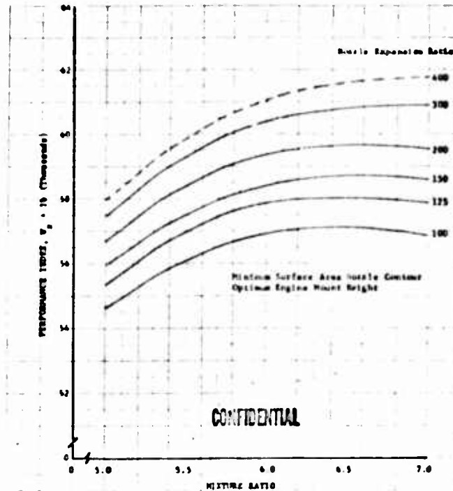
Figure 78. Performance Index vs Mixture Ratio for Case 6, 350K Module ( \epsilon_M = 300 ) DF 57638
