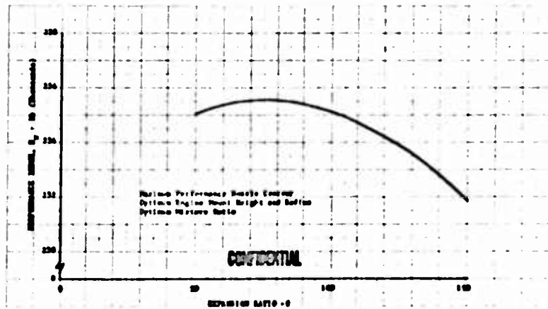
Figure 44. Performance Index vs Expansion Ratio for Case 1, 250K Module ( e_H = 250 ) DF 57551
