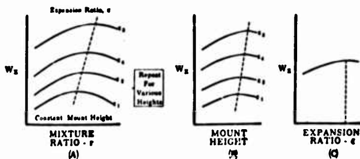
Figure 1. Optimization Procedure for an Upper Stage Case
