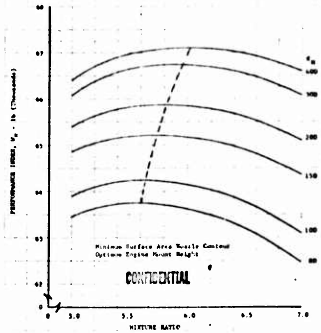
Figure 21. Performance Index vs Mixture Ratio for Case 2, 250K Module DF 57533
