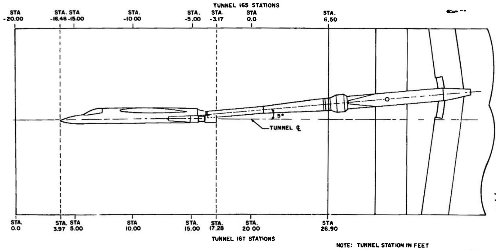
Fig. 1 Location of AMSA 1/8-Scale Inlet Model in Tunnel 16T and Tunnel 16S Test Sections
