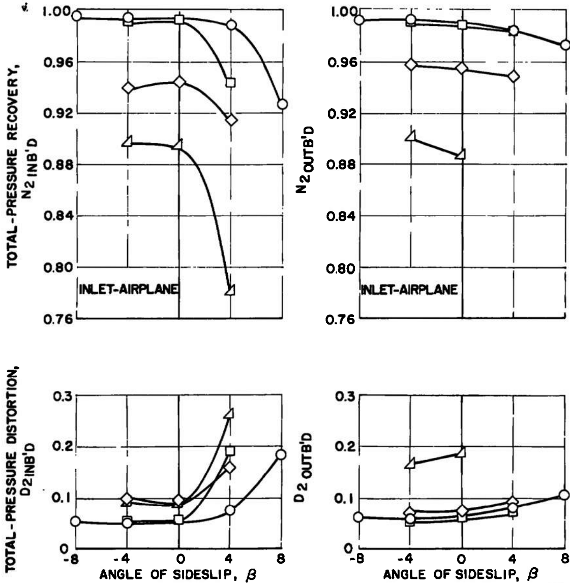
Fig. 18 Effect of Angle of Sideslip on Inlet Performance; \alpha = 6.2 deg
