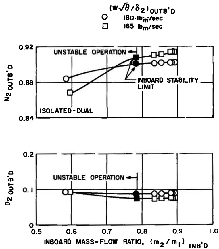
Fig. 14 (8) Mutual Interference Effect of Staggered Dual-Inlet Orientation on Inlet Performance; l_1^{27} Spike, M_\infty = 2.06 , \alpha = 0 deg, \beta = 0 deg, (X/R)_{INB'D} = 1.63 , (X/R)_{OUTB'D} = 1.67
