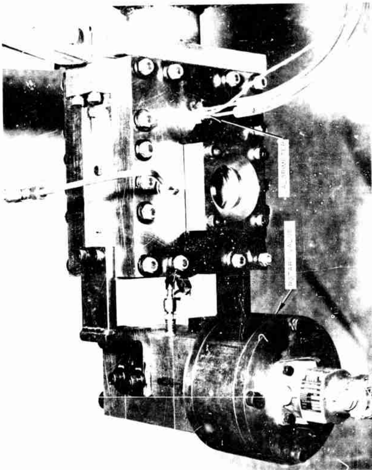
Figure 12 Photo of Rotary Valve Assembly Mounted to Combustor
