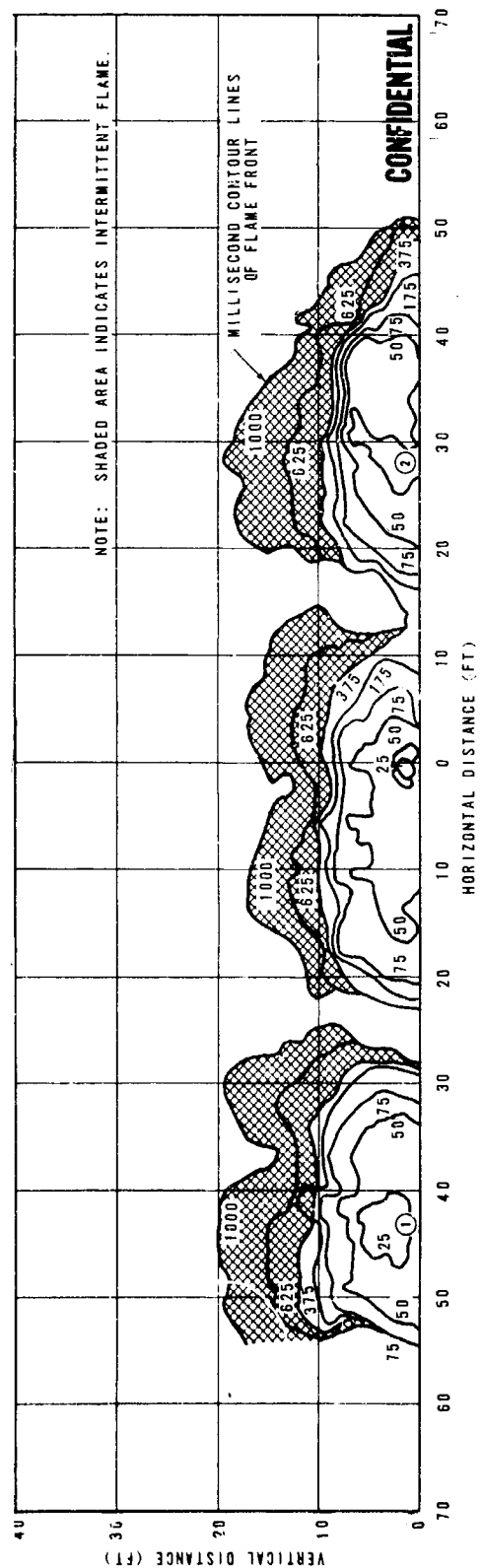
Figure 12. Fireball Propagation of Three Munitions Fired Simultaneously, View 1 (Frontal View).
