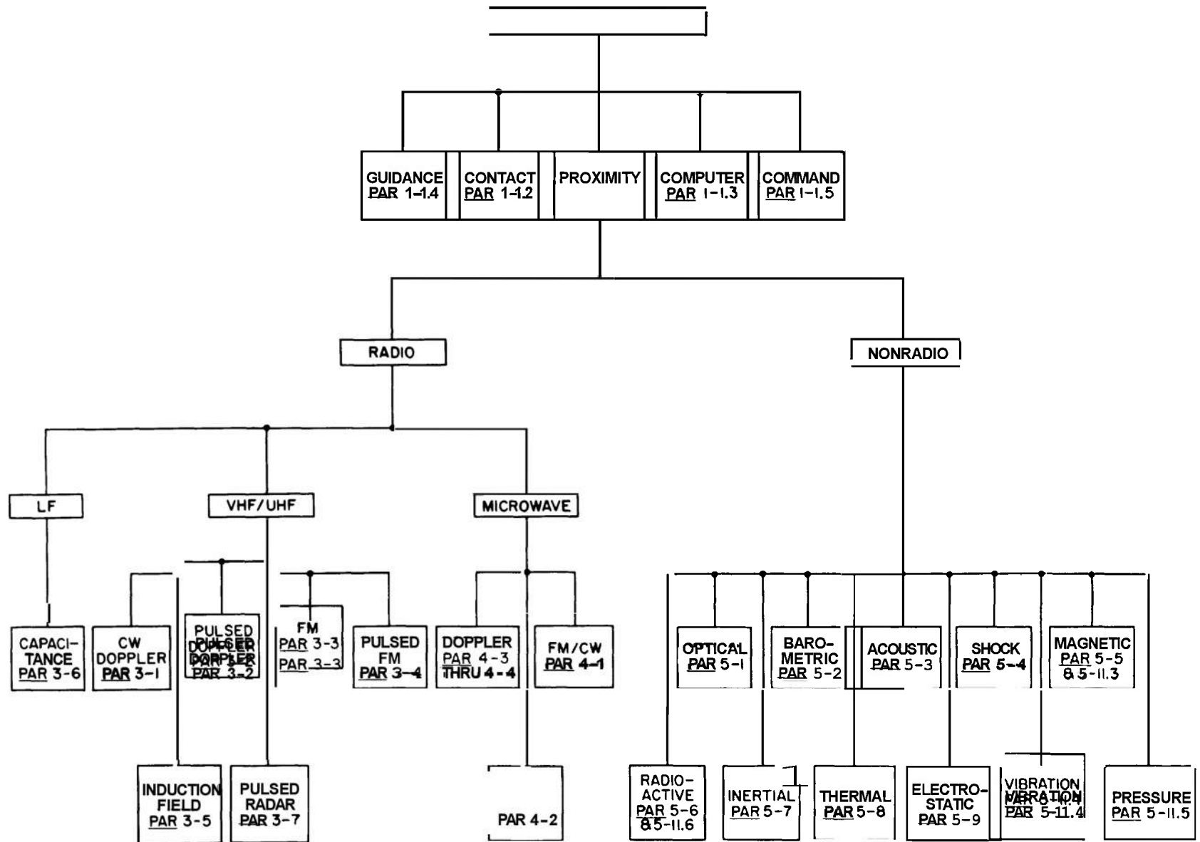
Figure I-1 (C). Types of Electrical Fuzes (U)
