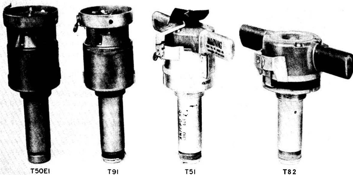
Figure 1-3 (U). Typical Bomb Fuzes Developed During World War II
