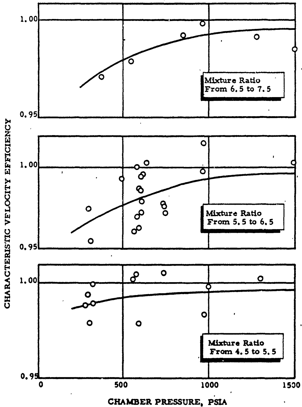
Figure 1. Triplet Injector Performance in the 2.5K Segment Thrust Chamber
