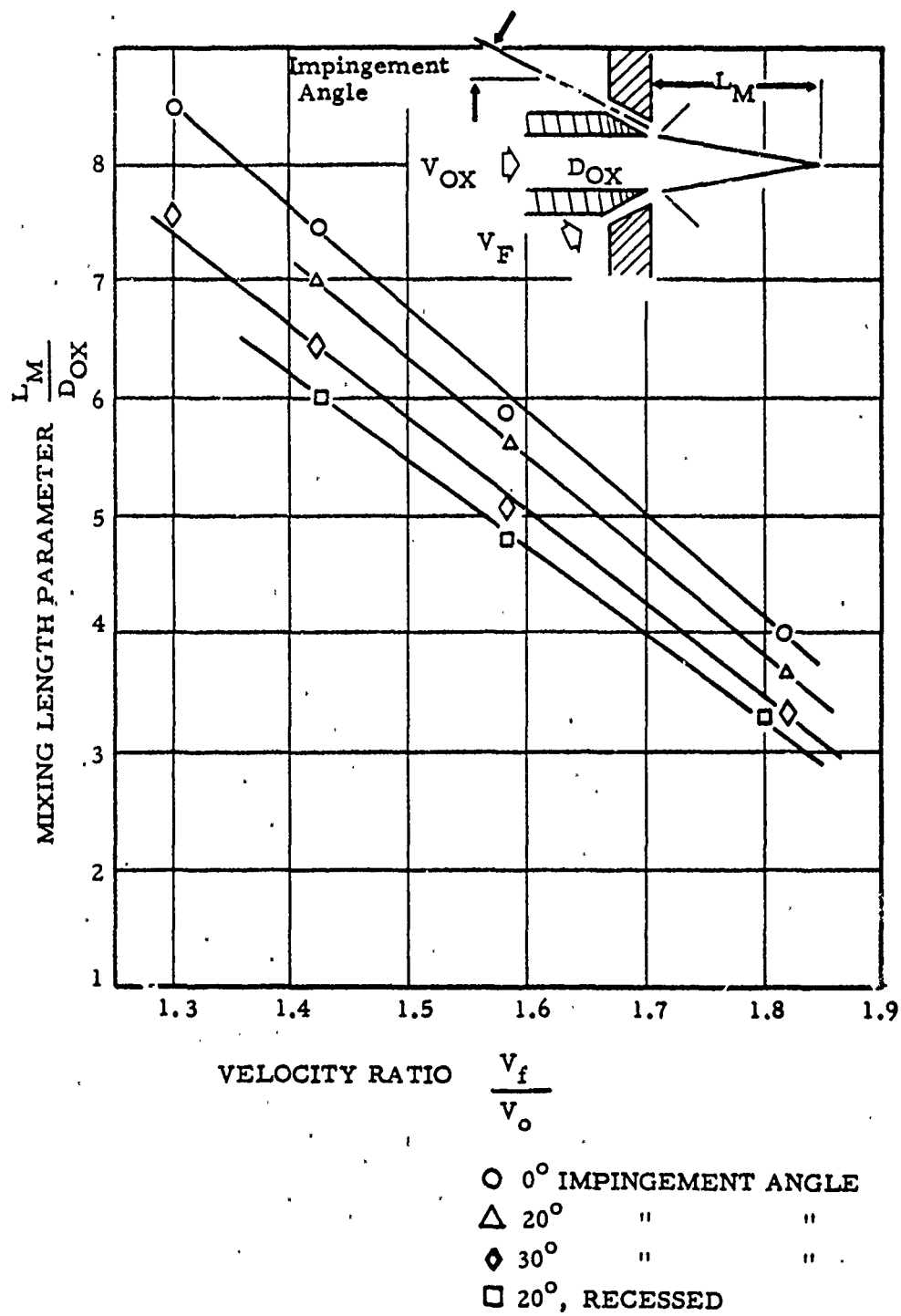
Figure 1. Coaxial Element Mixing Tests
