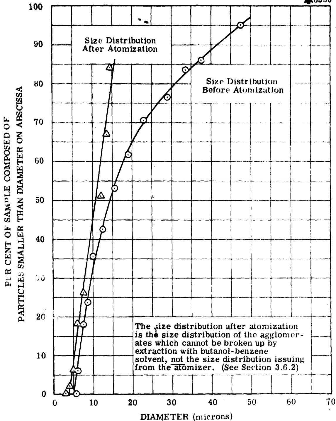
Figure 23. Comparison of Primary Agglomerate Size Distribution Present in Slurry of 75 Per Cent Ball-Milled Boron in Isopropanol Before and After Atomization by a Poppet Atomizer.
