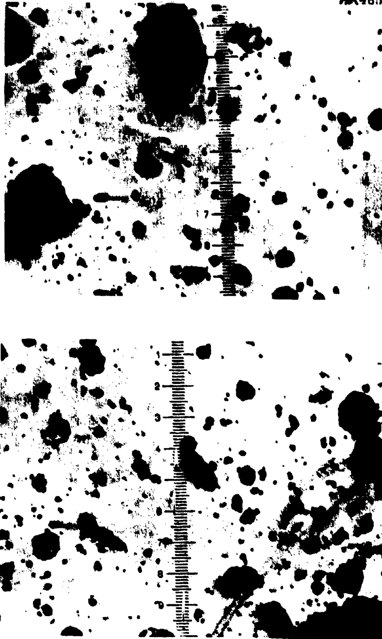
Figure 10. Photomicrographs of Atomized Boron Slurry (73 Per Cent Solids in JP-4) Collected, After Breakup by Particle Mill (Air Temperature 600°F, Air Flow Rate 0.2 lb/sec, Slurry Flow Rate 0.2 lb/sec), on a Greased Slide.
