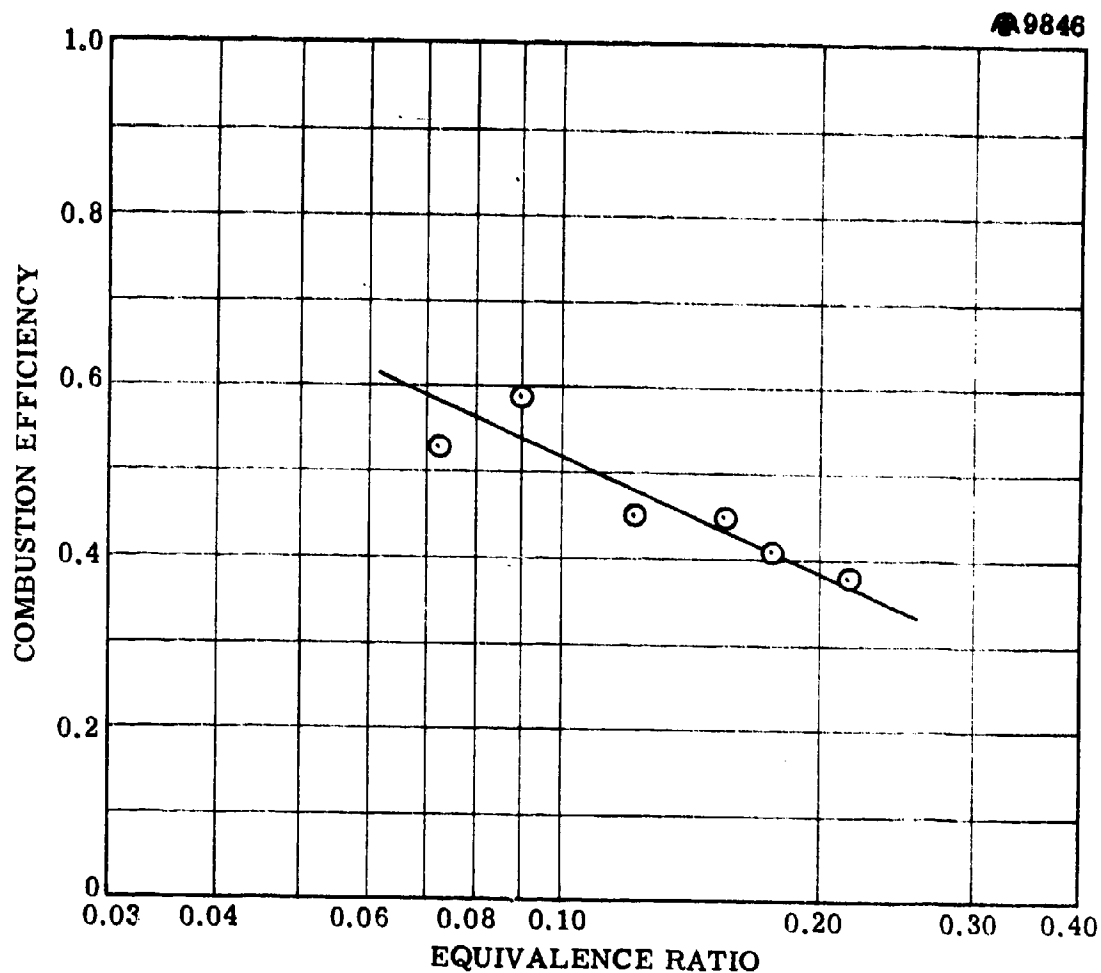
Figure 75. Combustion Efficiency Versus Equivalence Ratio for Test No. 13, using a JP-4 Based Boron Slurry Containing 73 Per Cent Solids Tested in the 3.5-inch Micro-Ramjet Engine Equipped with the Total Pressure Rake. Inlet Conditions - Mach 2.5 at Sea Level, Cold Day.
