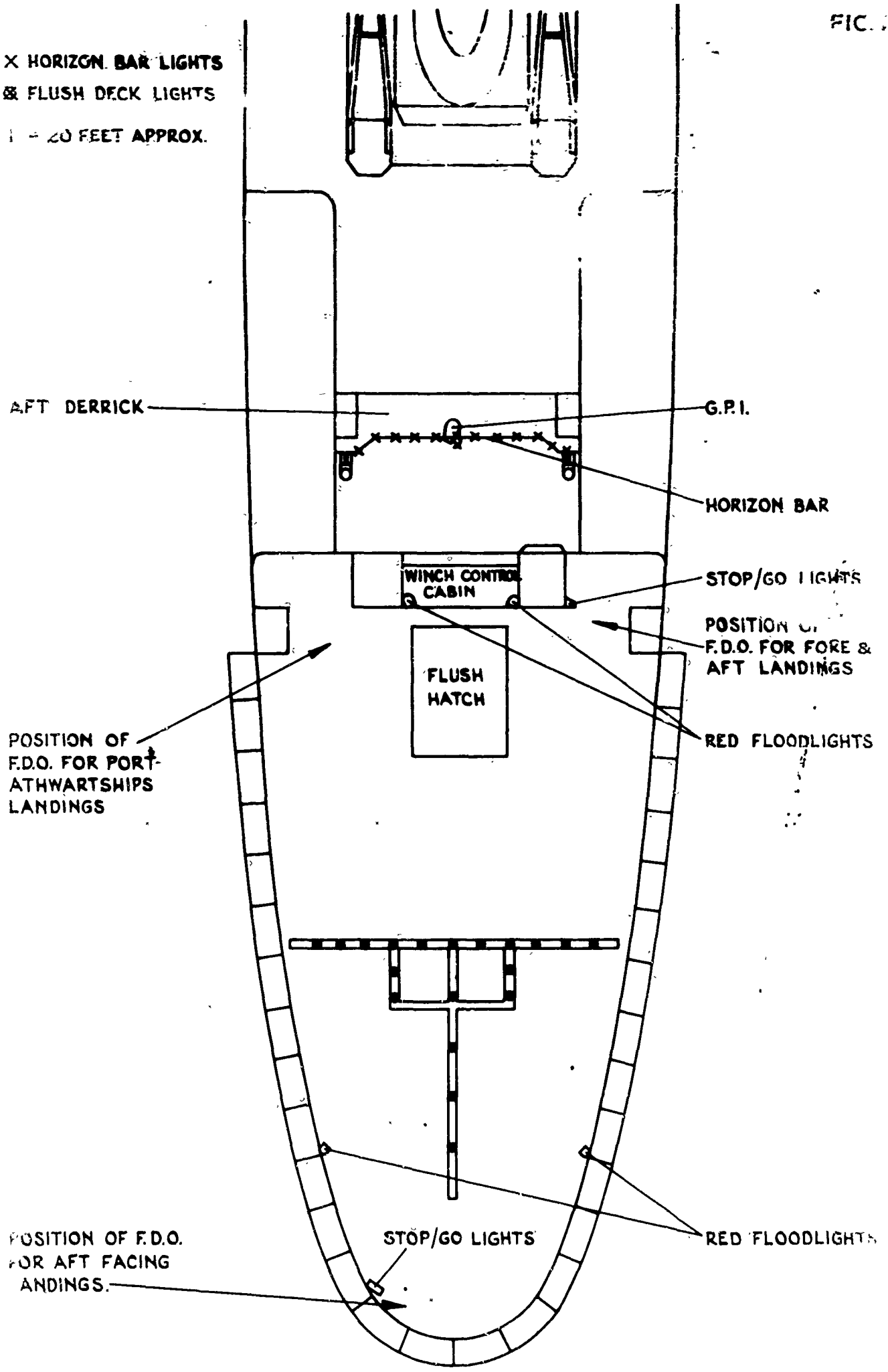
A SKETCH OF THE LAYOUT AND POSITION OF THE APPROACH AND LANDING AIDS OF R.F.A. LYNESS
