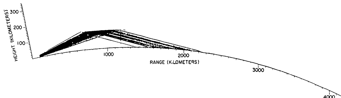
Fig. 19a - Ionospheric ray plot for ETR launch 3670, E-layer propagation
