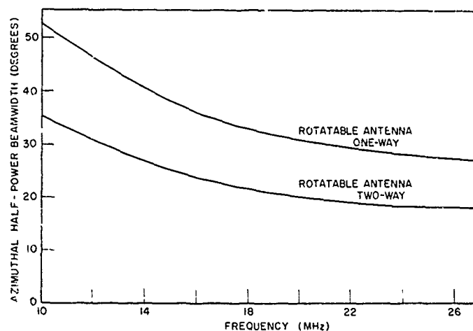
Fig. 5 - Azimuthal half-power beamwidth vs frequency for the rotatable antenna
