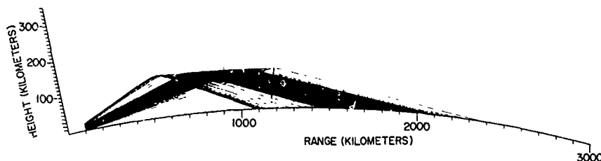
Fig. 52 - Ionospheric ray plot for the ETR launch 2949
