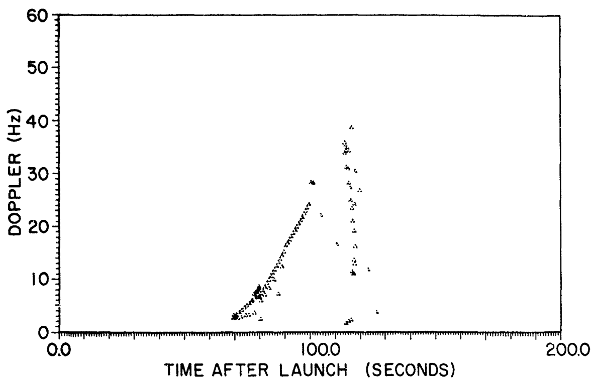
Fig. 35b - Simulated signature for ETR launch 0038, F-layer contribution
