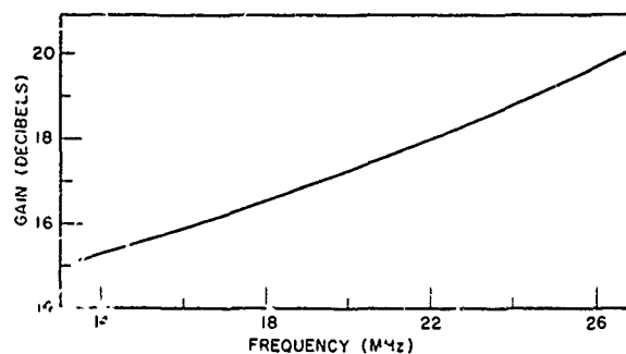
Fig. 2 - Estimated effective gain vs frequency for the rotatable antenna's principal lobe (including an assumed 5-dB ground enhancement)
