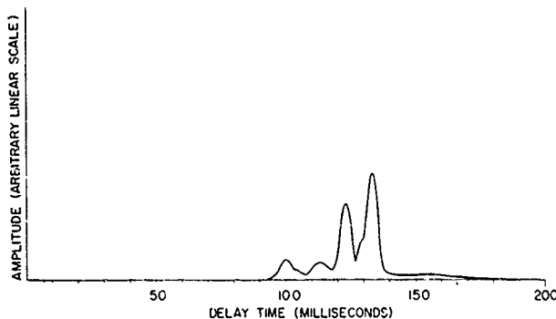
Fig. 44 - Predicted ground-backscatter distribution for the ETR launch 4941
