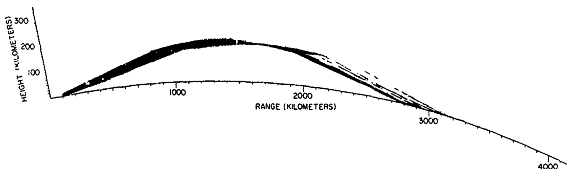
Fig. 19b - Ionospheric ray plot for ETR launch 3670, F-layer propagation
