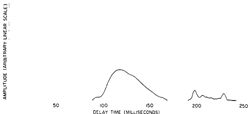
Fig. 20 - Predicted ground-backscatter distribution for ETR launch 3670 with the E- and F-layer contributions superimposed
