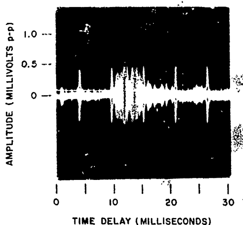
Fig. 8 - Observed ground-backscatter distribution, 1425 EST, May 25, 1964 ETR launch 2955
