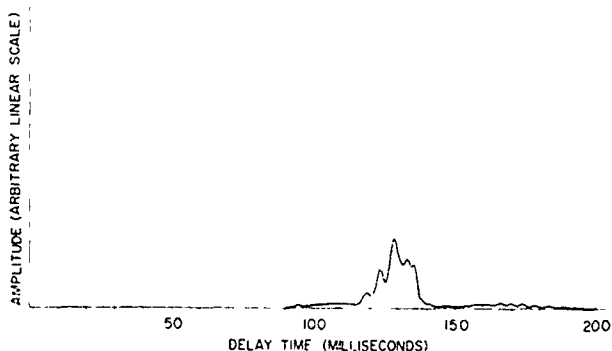
Fig. 10 - Predicted ground-backscatter distribution for ETR launch 2955
