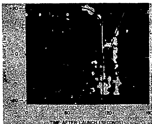
Fig. 12 - Observed signature for ETR launch 2955
