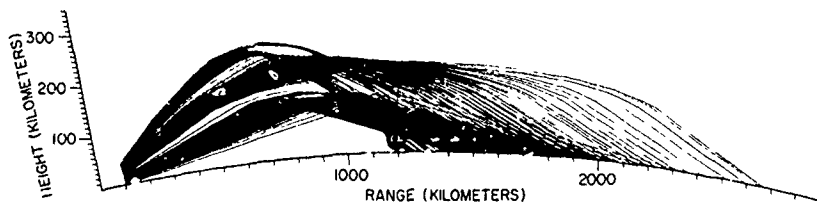
Fig. 28 - Ionospheric ray plot for ETR launch 0324
