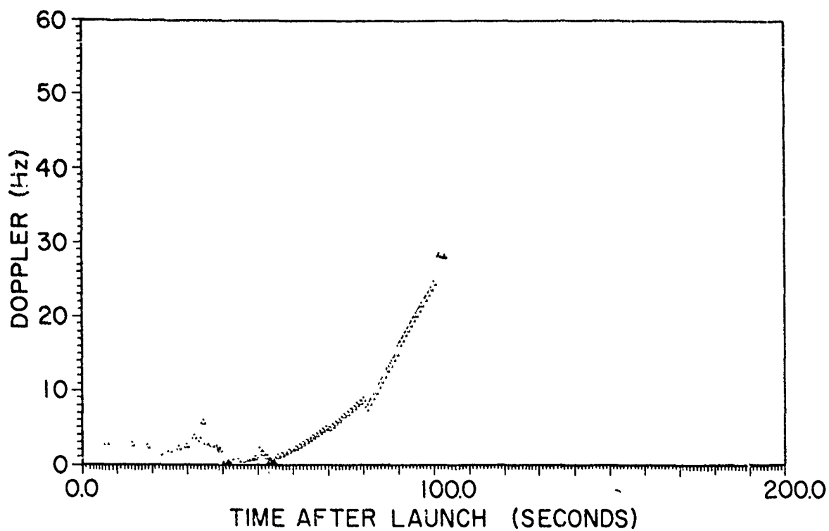
Fig. 35a - Simulated signature for ETR launch 0038, E-layer contribution
