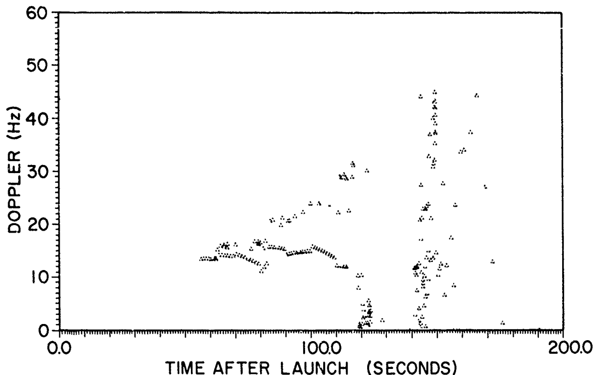
Fig. 45 - Simulated signature for the ETR launch 4941
