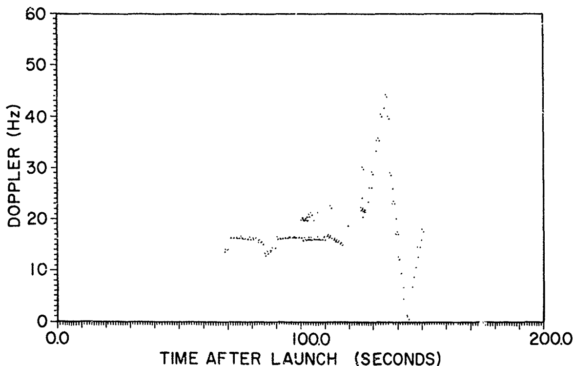
Fig. 16 - Simulated signature for ETR launch 2903
