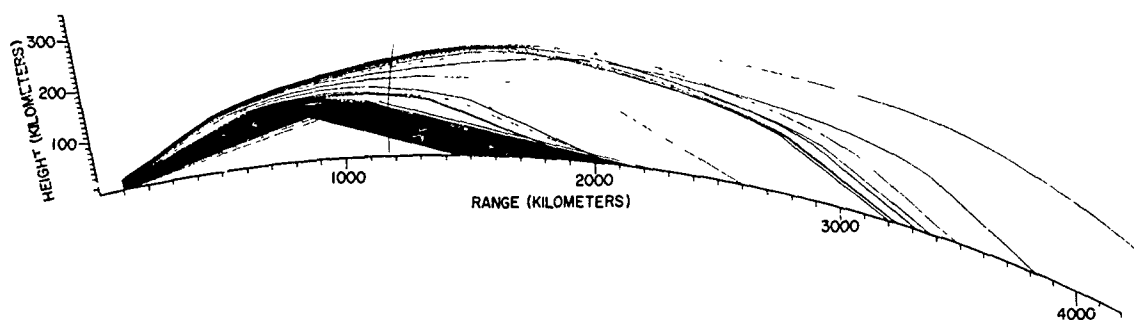
Fig. 14 - Ionospheric ray plot for ETR launch 2903
