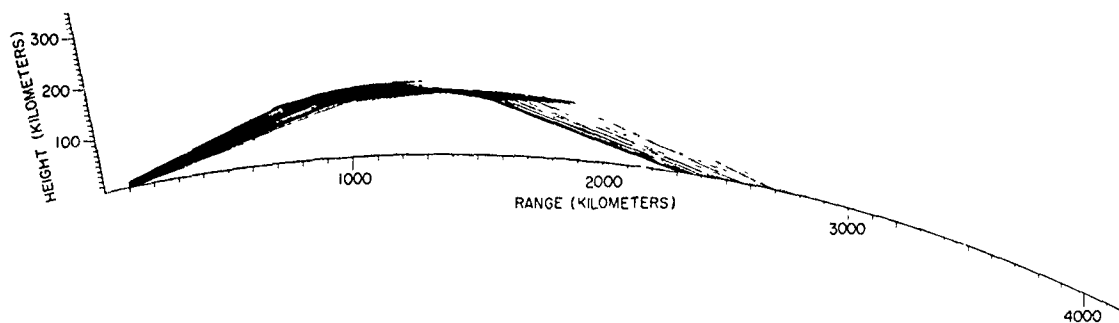
Fig. 23b - Ionospheric ray plot for ETR launch 3688, F-layer propagation
