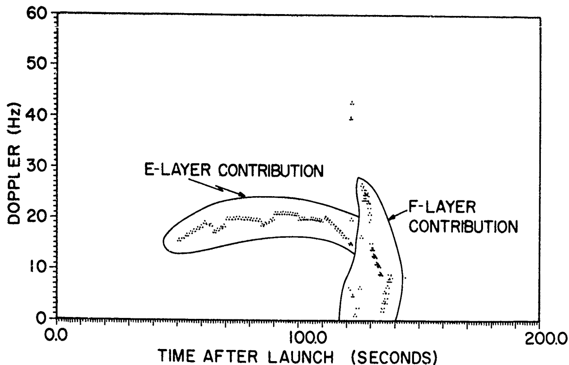
Fig. 21 - Simulated signature for ETR launch 3670 with the E- and F-layer contributions superimposed
