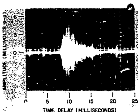
Fig. 27 - Observed ground-backscatter distribution, 1225 EST, Jan. 20, 1964, ETR launch 0324
