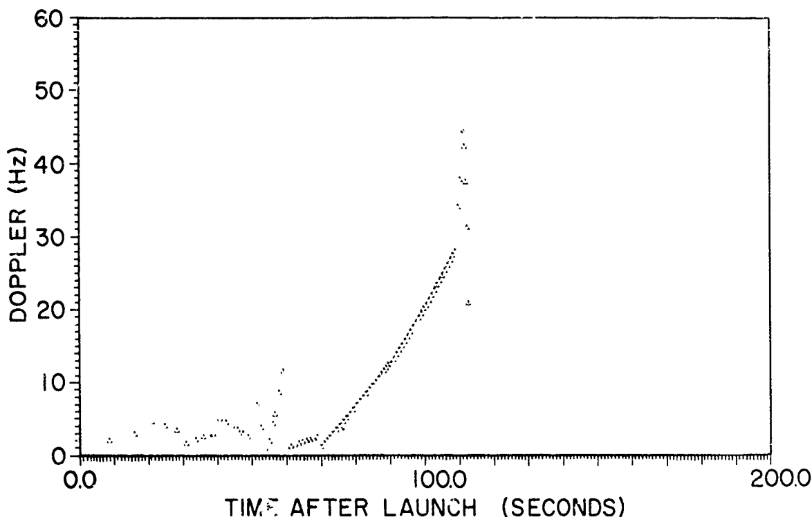
Fig. 54 - Simulated signature for the ETR launch 2949
