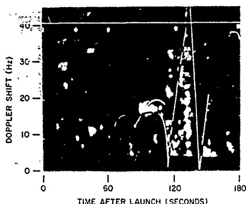
Fig. 17 - Observed signature for ETR launch 2903
