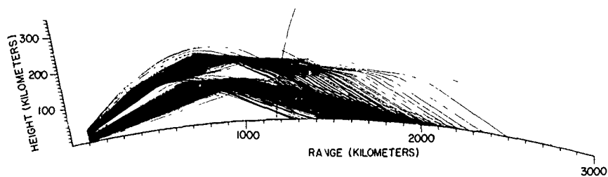
Fig. 38 - Ionospheric ray plot for ETR launch 0303
