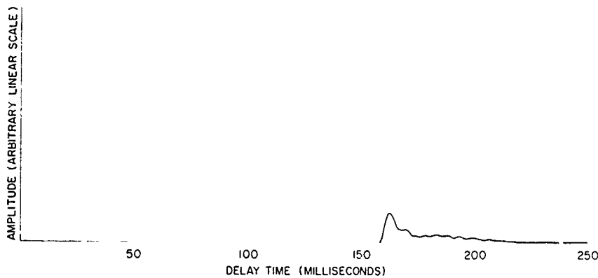
Fig. 24b - Predicted ground-backscatter distribution for ETR launch 3688; F-layer contribution
