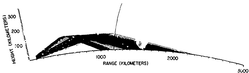
Fig. 33a - Ionospheric ray plot for ETR launch 0038, E-layer propagation
