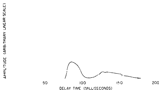
Fig. 49 - Predicted ground-backscatter distribution for the ETR launch 0238
