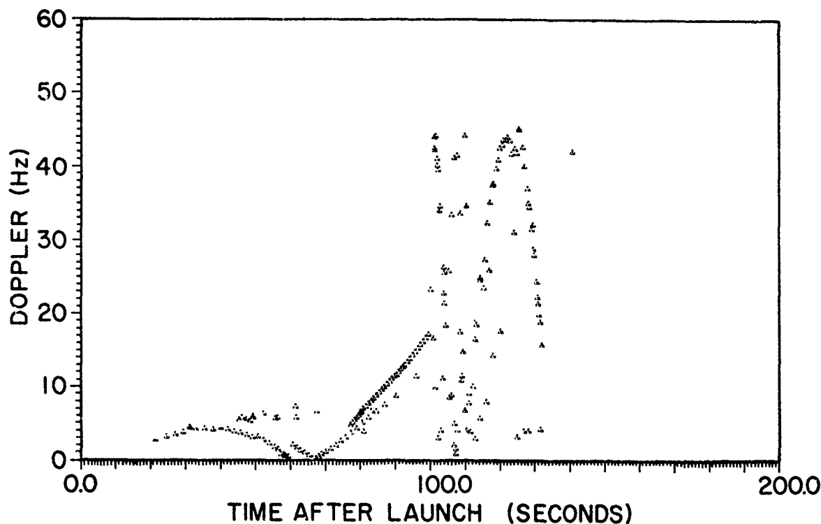
Fig. 40 - Simulated signature for the ETR launch 0303
