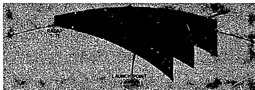
Fig. 7 - Perspective view of three adjacent vertical planes upon which ray trajectories are shown emanating from the radar site and intersecting the missile trajectory
