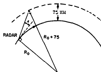
Fig. B2 - Ray geometry for D -layer absorption calculation
