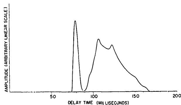
Fig. 53 - Predicted ground-backscatter distribution for the ETR launch 2949
