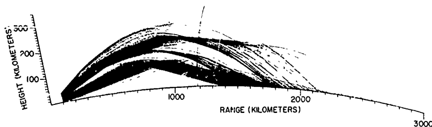
Fig. 43 - Ionospheric ray plot for the ETR launch 4941
