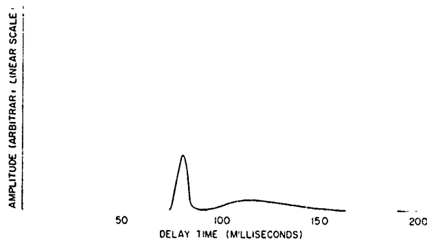
Fig. 24a - Predicted ground-backscatter distribution for ETR launch 3688; E-layer contribution
