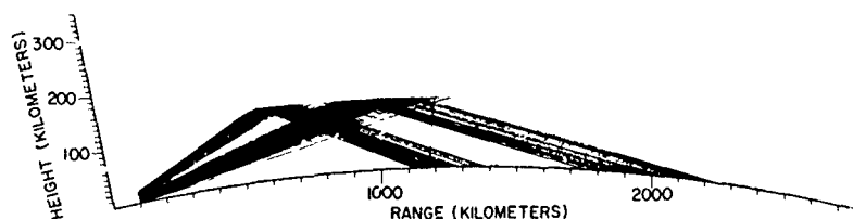
Fig. 46 - Ionospheric ray plot for the ETR launch 0238
