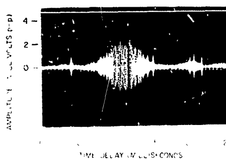
Fig. 37 - Observed ground-backscatter distribution (near launch time) on Jan. 26, 1964 for the ETR launch 0303
