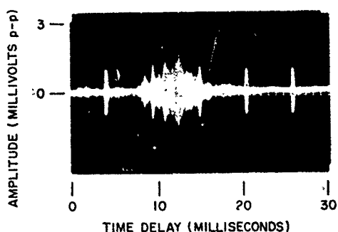
Fig. 42 - Observed ground-backscatter distribution at 1105 EST on Sept. 28, 1964 for the ETR launch 4941
