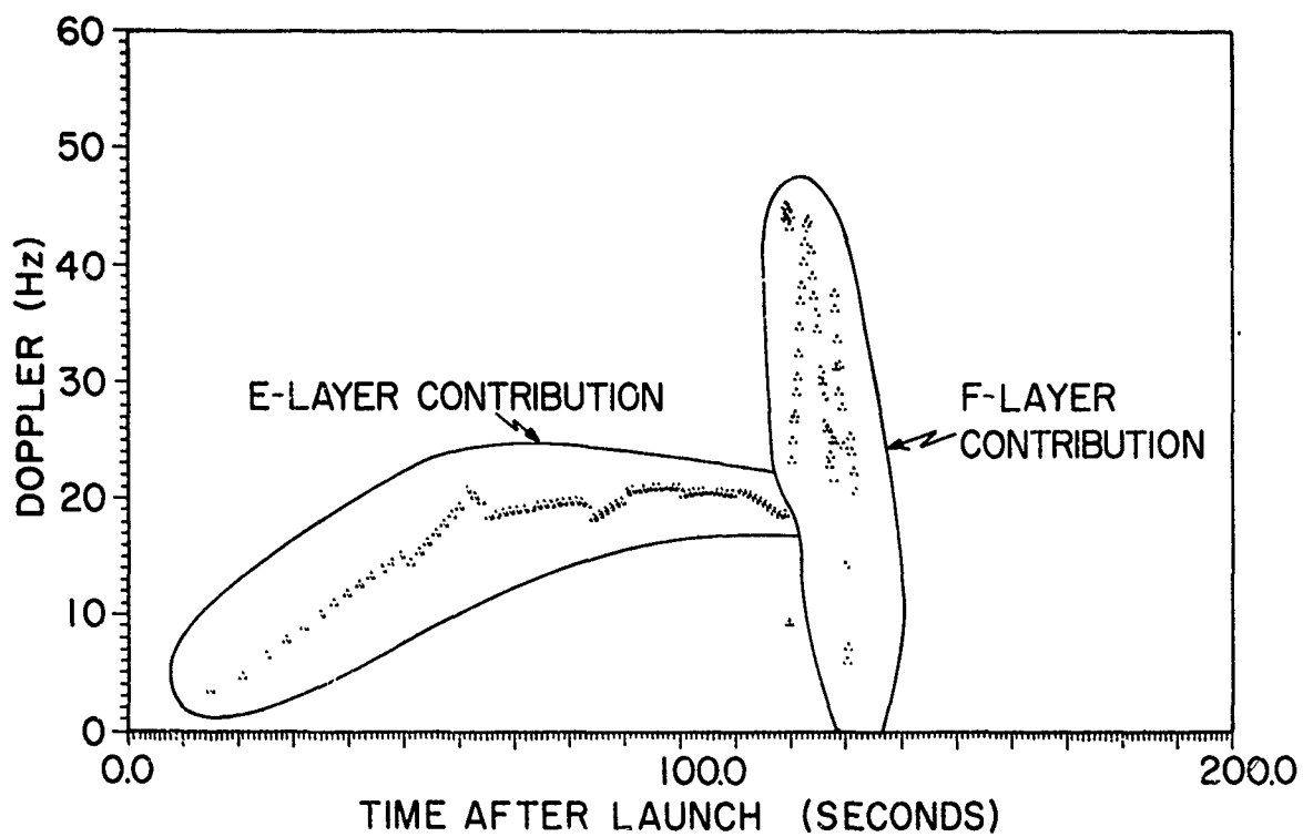
Fig. 25 - Simulated signature for ETR launch 3688. The E- and F-layer contributions are superimposed.
