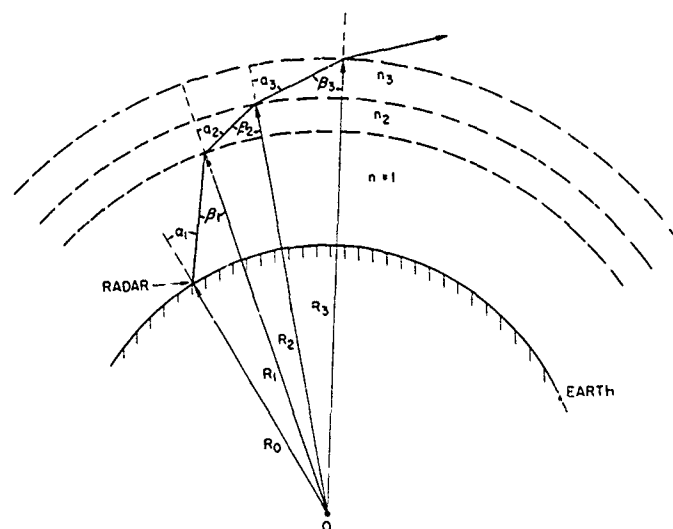
Fig. A1 - Ionospheric refraction geometry for the ray-tracing computer program
