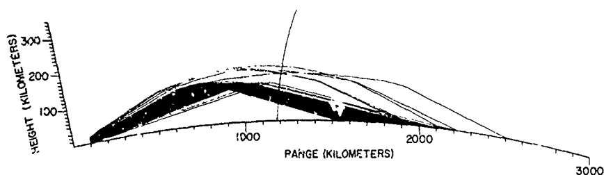
Fig. 33b - Ionospheric ray plot for ETR launch 0038, E- and F-layer propagation
