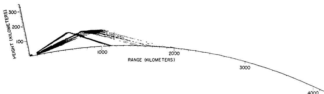
Fig. 23a - Ionospheric ray plot for ETR launch 3688, E-layer propagation
