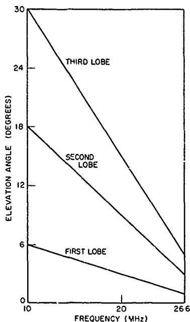
Fig. 3 - Lobe elevation vs center frequencies for the rotatable antenna
