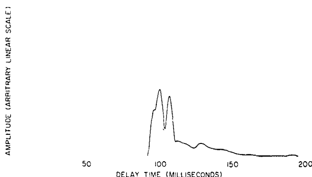
Fig. 29 - Predicted ground-backscatter distribution for ETR launch 0324
