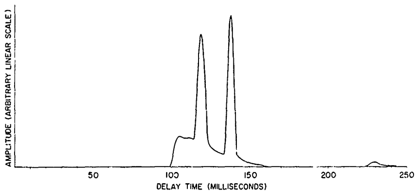
Fig. 15 - Predicted ground-backscatter distribution for ETR launch 2903
