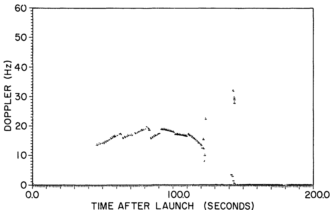
Fig. 11 - Simulated signature for ETR launch 2955
