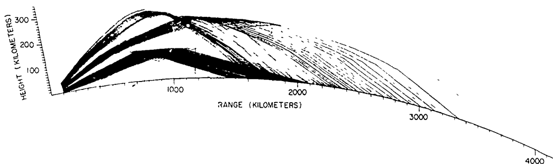
Fig. 9 - Ionospheric ray plot for ETR launch 2955
