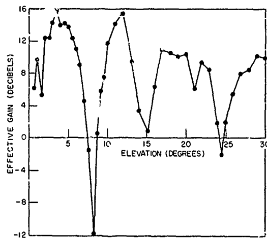
Fig. 4 - Measured elevation-plane pattern of the rotatable antenna at 15.6 MHz, with the antenna oriented in a southerly direction
