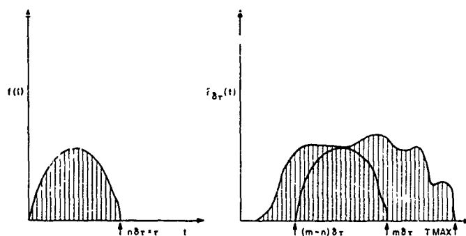
Fig. B3 - Illustration of the use of convolution to yield the amplitude of the received ground-backscattered energy due to an illuminating pulse of arbitrary pulse-shape
