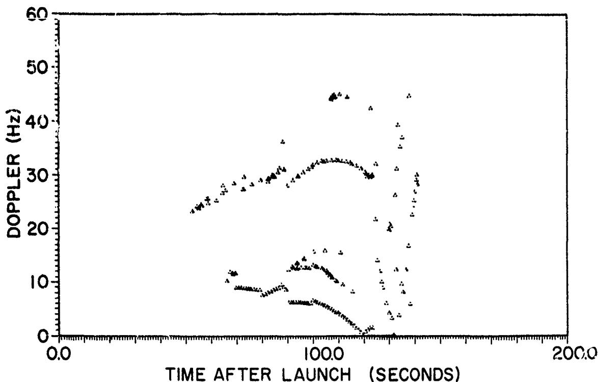
Fig. 30 - Simulated signature for ETR launch 0324
