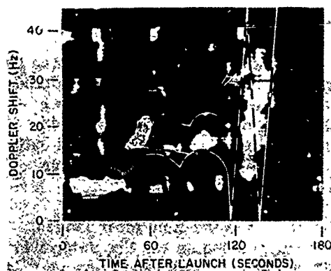
Fig. 46 - Observed signature for the ETR launch 4941
