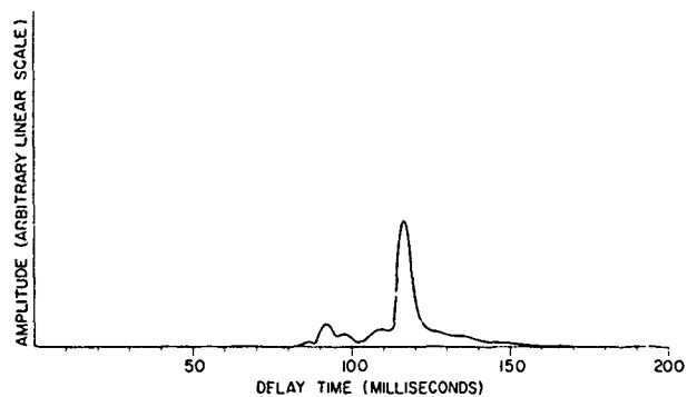
Fig. 39 - Predicted ground-backscatter distribution for the ETR launch 0303
