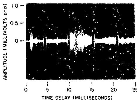
Fig. 18 - Observed ground-backscatter distribution, 1050 EST, July 30, 1964, ETR launch 3670
