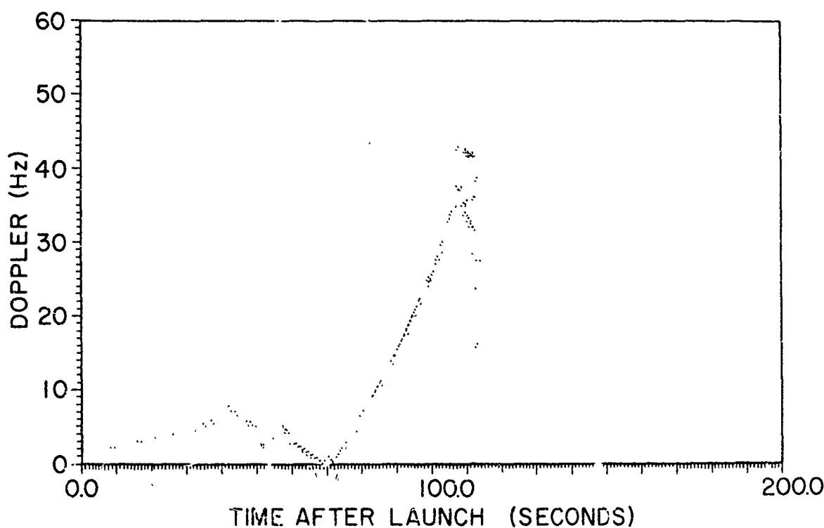
Fig. 50 - Simulated signature for the ETR launch 0238
