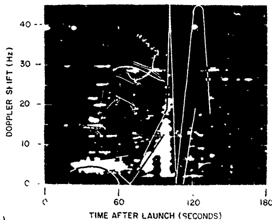
Fig. 41 - Observed signature for the ETR launch 0303
