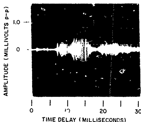
Fig. 47 - Observed ground-backscatter distribution at 1040 EST on Feb. 3, 1964 for the ETR launch 0238
