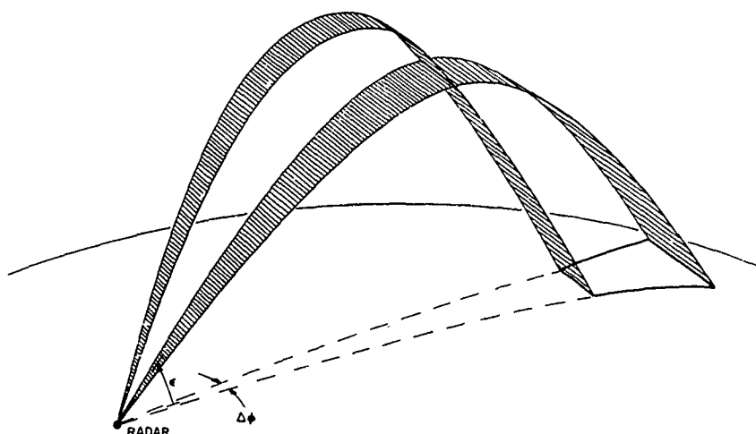
Fig. B1 - Sketch of a flux tube of elevation \epsilon and azimuthal angular width \Delta\phi between the radar transmitter and the earth after an ionospheric traversal
