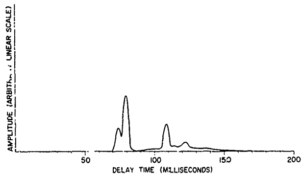
Fig. 34 - Predicted ground-backscatter distribution for ETR launch 0038 with the E- and F-layer contributions superimposed
