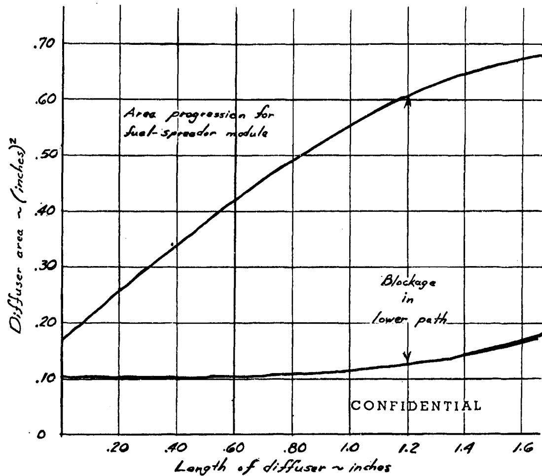
Figure 17. Diffuser area versus length of diffuser "D"-diffuser, fuel-air spreader module, lower path.
