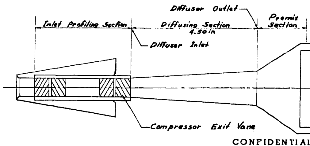
Figure 20. Combustion rig "A" diffuser flow path.
