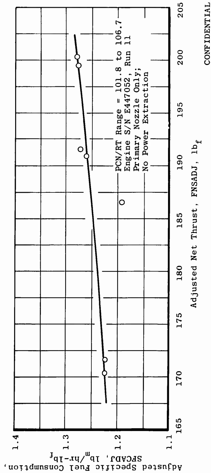
(C) Fig. 11 Specific Fuel Consumption as a Function of Net Thrust at N = 5000 \text{ ft} , Mach Number 0.85
