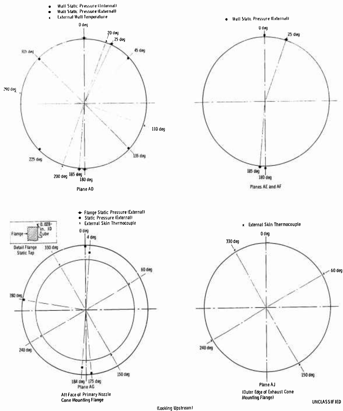
d. Primary Exhaust Nozzle Cone Fig. 5 Continued
