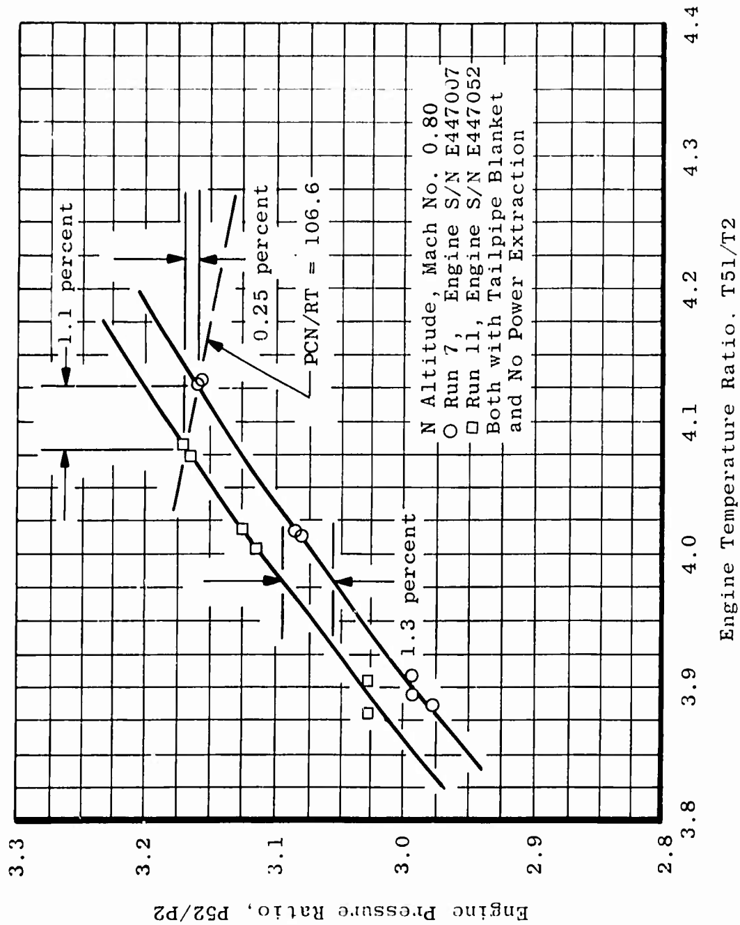
(U) Fig. 9 Comparison of Pumping Characteristics of J97 Engines S/N E447007 and E447052
