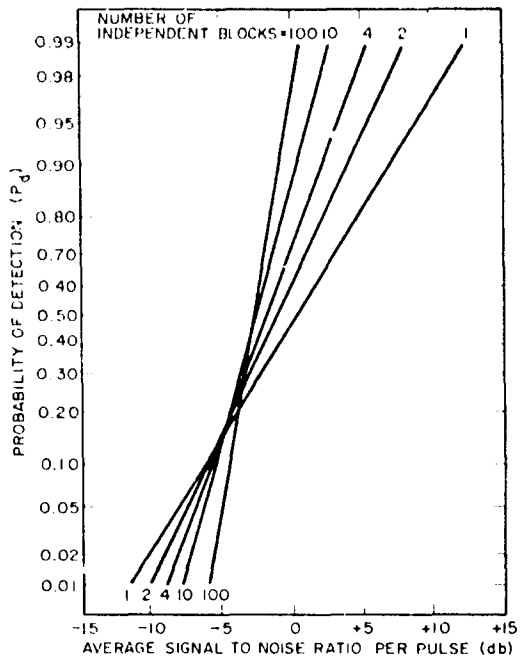
Fig. 7 - Radar detection probability for log-normally distributed targets ( \sigma = 3 ; \lambda = 100 ; probability of a false alarm P_{fa} = 10^{-6} )
