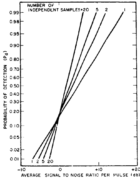
Fig. 9 - Radar detection probability for log-normally distributed targets ( \sigma = 2 , \lambda = 20 ; probability of a false alarm P_{fa} = 10^{-3} )
