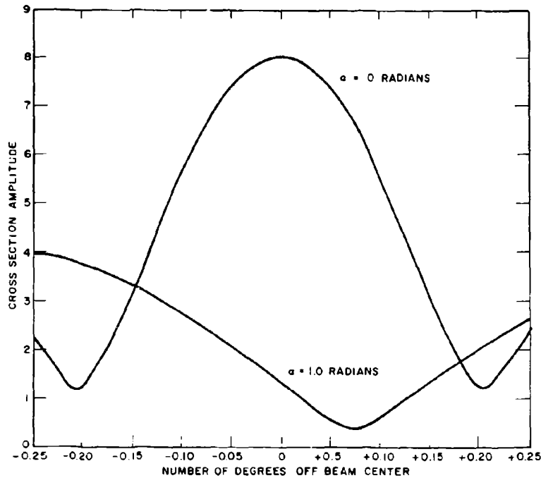
Fig. 3 - Returned signal from a fluctuating target ( L = 100 ft; \lambda = 1.0 ft; N = 8 ; \sigma = 0.5 degree)
