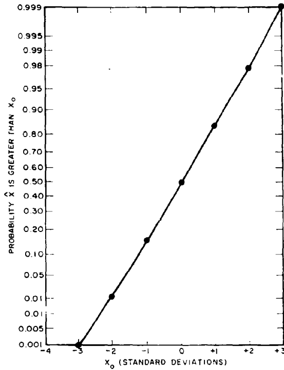
Fig. 15 - Distribution of \hat{x} - IMA
