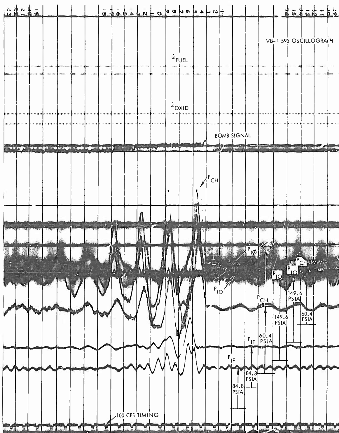
Figure 26. VBI-595 Oscillograph (No. 1) from Before Charge Detonation to 150 msec After Detonation
