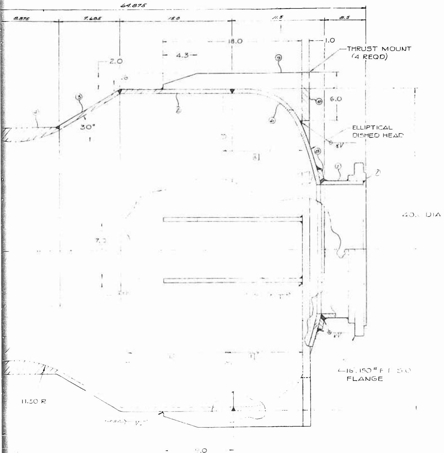
Figure 6. Combustion Chamber 250,000 lb f Thrust, Static Test Engine (SK 401379 JC-1)
