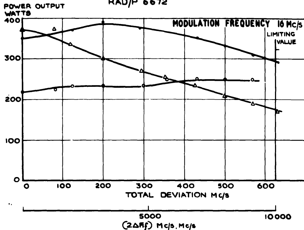
FIG. 13 VX 3510/CV2470 (2500-3100 Mc/s) VARIATION OF OUTPUT POWER WITH DEVIATION AND (2\Delta Ff)
