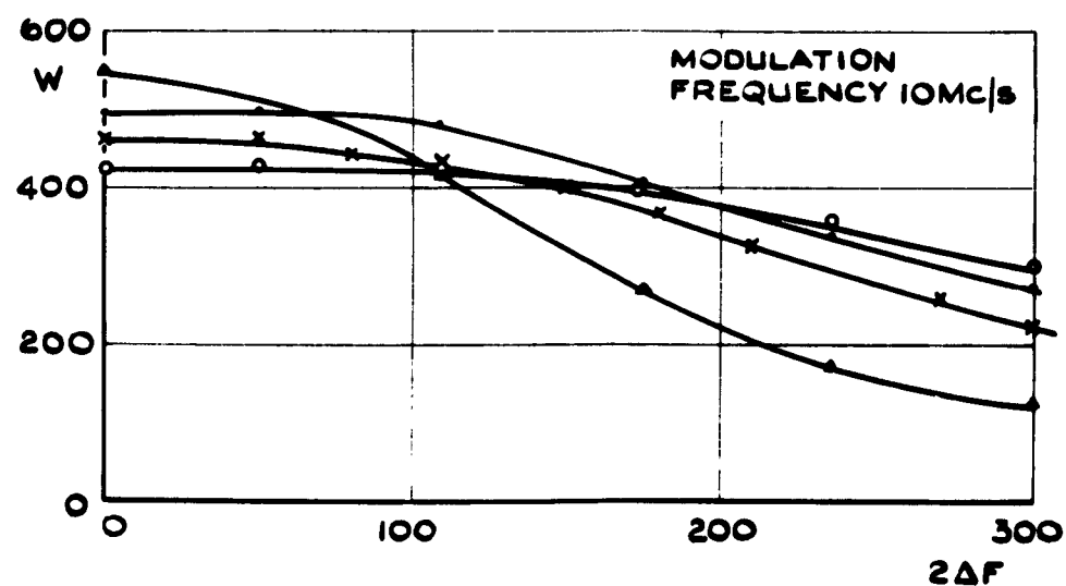
FIG.11 VX 9240 (1060-1370 Mc/s) VARIATION OF OUTPUT POWER WITH MODULATING FREQUENCY AND DEVIATION
