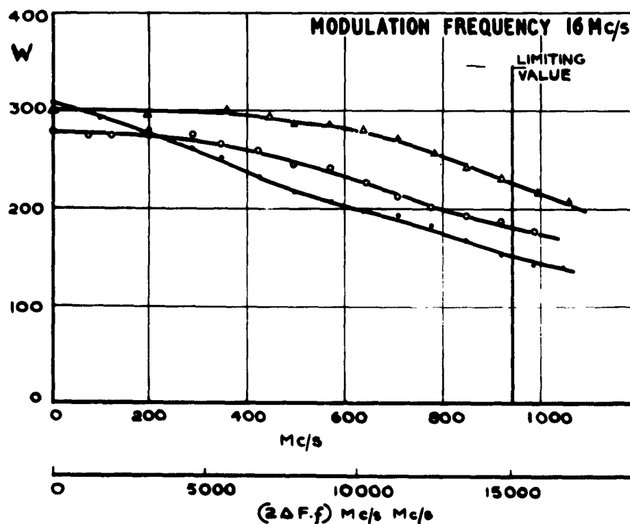
FIG. 14 VX 3512/CV 2471 (3000-4000 Mc/s) VARIATION OF OUTPUT POWER WITH DEVIATION AND (2\Delta Ff)
