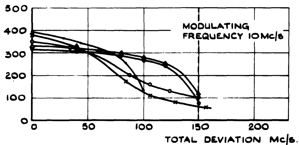
FIG.4 VX 9224/CV 6102 (520-670 Mc/s) VARIATION OF OUTPUT POWER WITH MODULATING FREQUENCY AND DEVIATION
