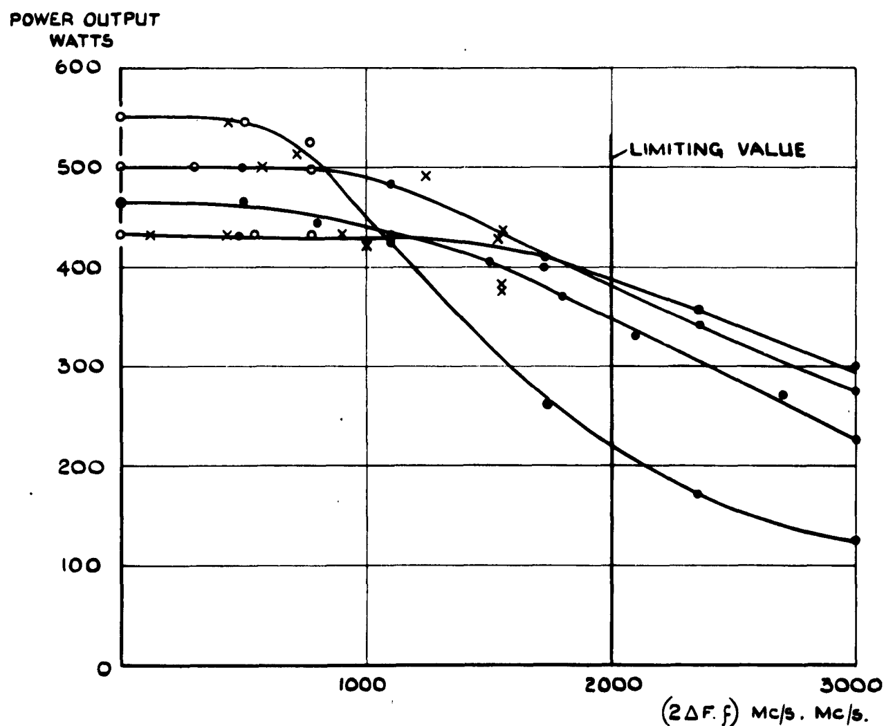
FIG.12 VX 9240 (1060-1370 Mc/s) VARIATION OF OUTPUT POWER WITH ( 2\Delta F. f ) FOR MODULATION FREQUENCY OF 2.5, 5, 10 Mc/s
