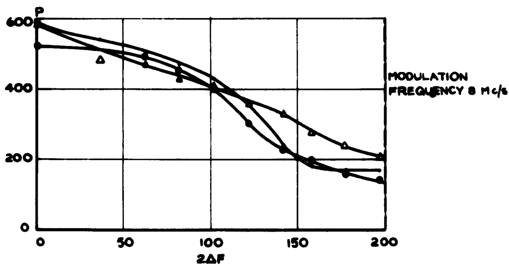
FIG 6 VX9239/CV6124 (6c VARIATION OF OUTPUT POWER WITH MODULATION
