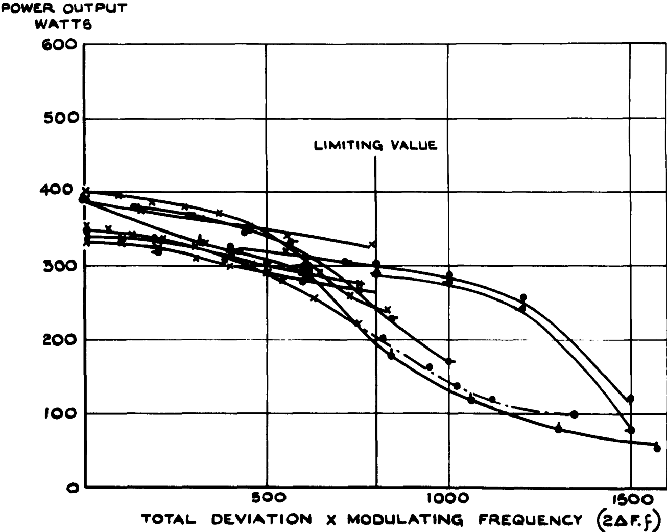
FIG.5 VX 9224/CV 6102 (520-670 Mc/s) VARIATION OF OUTPUT POWER WITH ( 2f \cdot \Delta f ) FOR f OF 5, 8, 10 Mc/s
