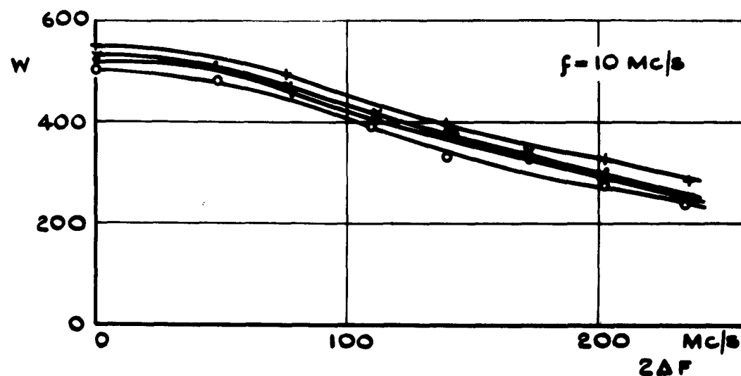
FIG.9 VX 9250 (850-1100 Mc/s) VARIATION OF OUTPUT POWER WITH MODULATING FREQUENCY AND DEVIATION
