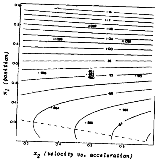
Figure 3 Tracking accuracy. Target crossing distance 5,000 ft. with 2g vertical weave. Contours are spaced at intervals of 0.02 log r.m.s. error.
