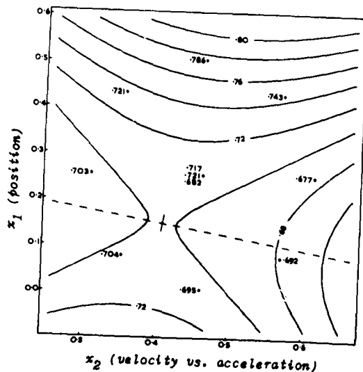
Figure 2 Tracking accuracy. Target crossing distance 2,500 ft. Contours are spaced at intervals of 0.02 log r.m.s. error.
