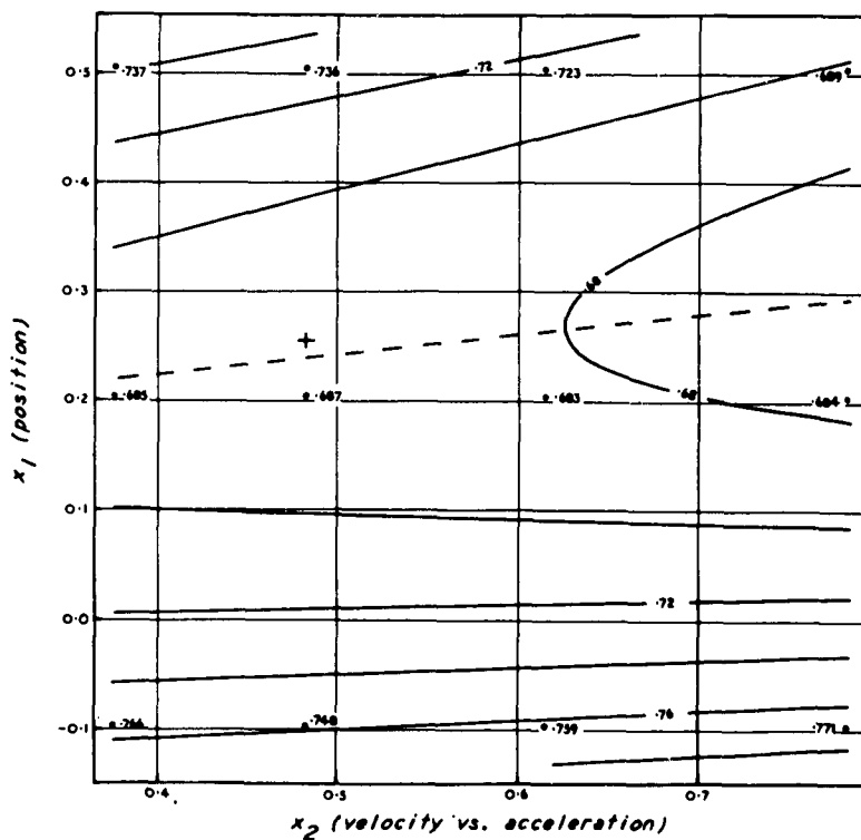
Figure A2 Tracking accuracy. Target crossing distance 2,500 ft. with 3g vertical weave. Contours are spaced at intervals of 0.02 log r.m.s. error. The point chosen as the centre for the main experiment design is marked by a vertical cross.
