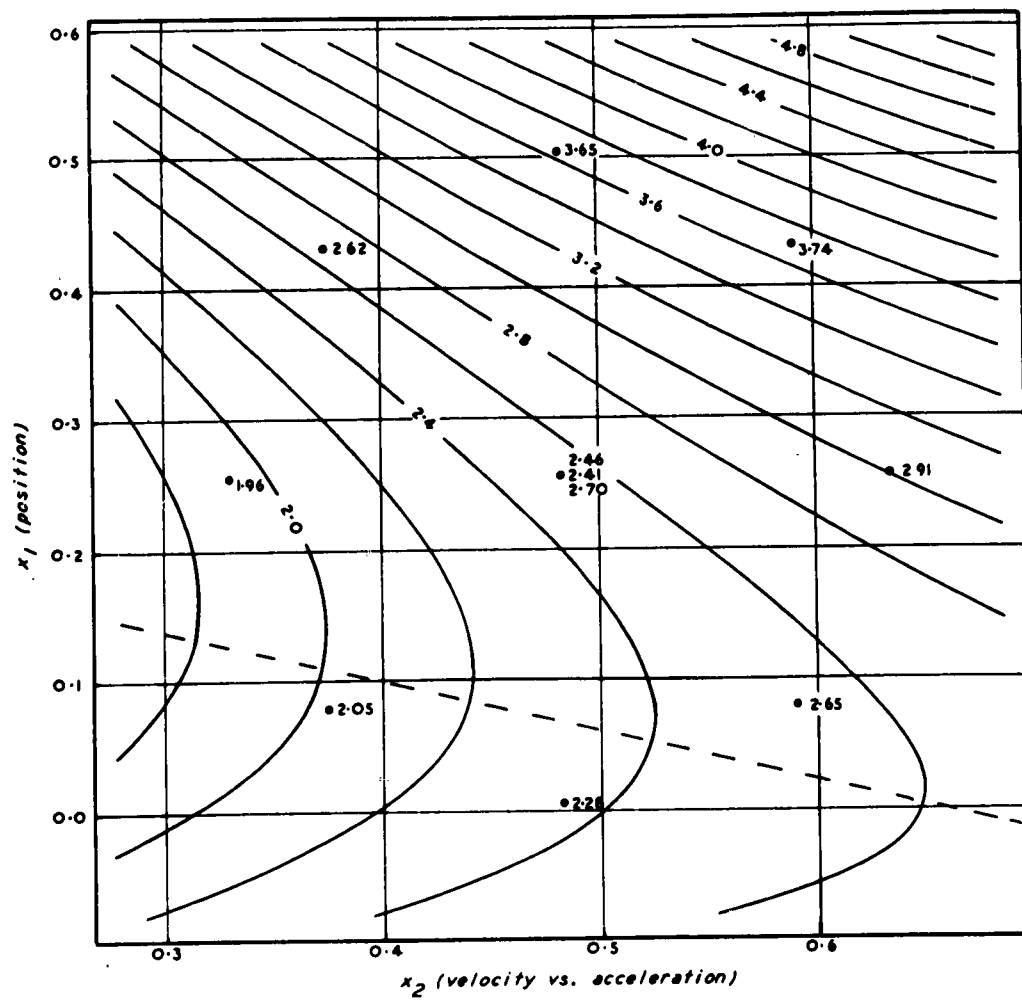
Figure 9 Acquisition and settling time. All three target courses pooled. Contours are spaced at intervals of 0.2 secs.
