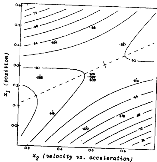
Figure 1 Tracking accuracy. Target crossing distance 10,000 ft. Contours are spaced at intervals of 0.02 log r.m.s. error.
