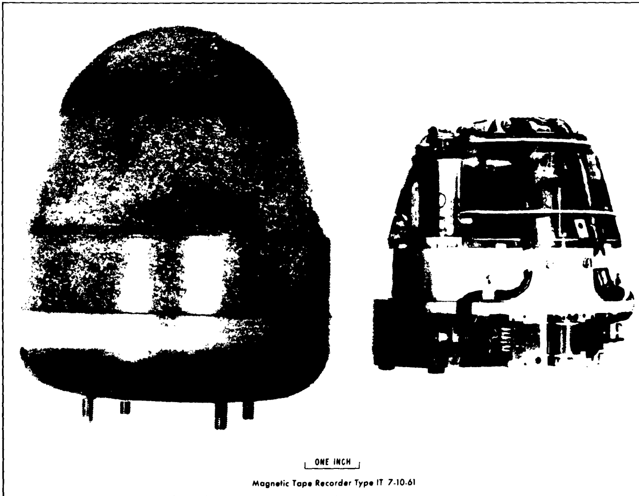
Fig.8 Long play tape recorder, and duresitos capsule
