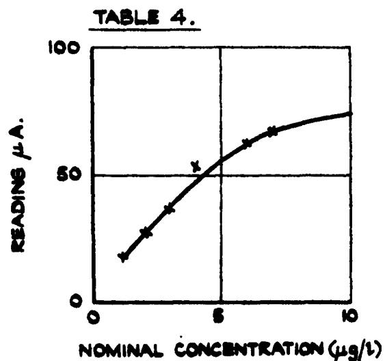
(f) DIMETHYLANILINE
