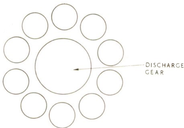
FIG. 2. 10 Tube arrangement.
