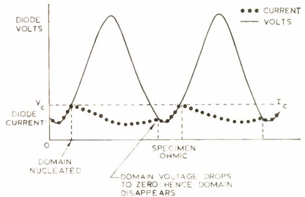
FIG. 7. Negative resistance modes (Quenched domain modes or L.S.A. modes).
