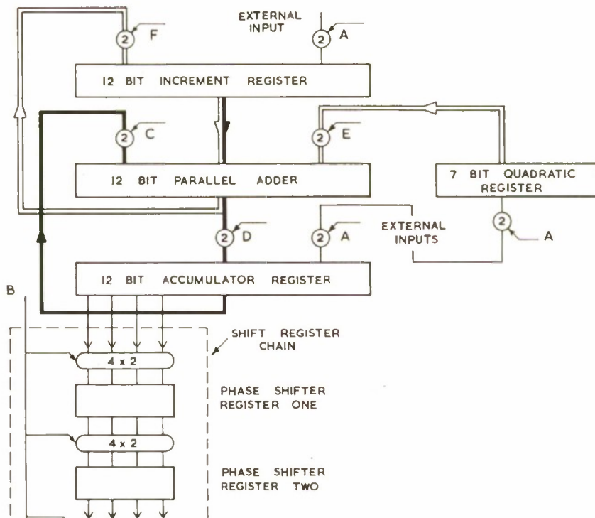
FIG. 6. Logic diagram for Control Circuits.
