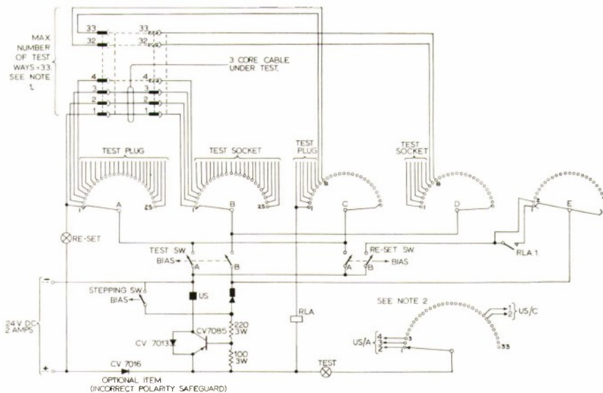
FIG. 2. Circuit diagram.
