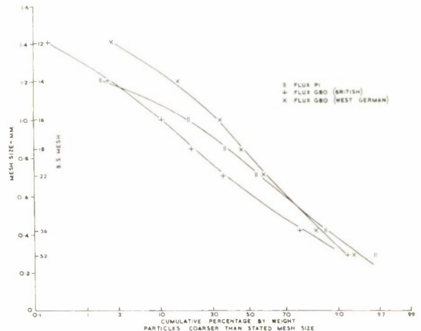
FIG. 11. Size distribution (cumulative) for commercial fused fluxes P1 and G80.
