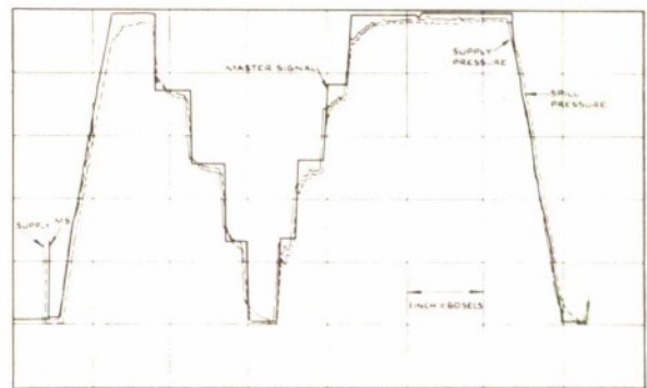
FIG. 8. Fuel system transient response.
