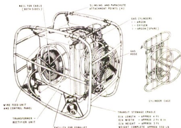
FIG. 16. Lightweight Field Welding Equipment.
