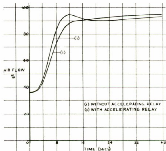
FIG. 11. Computed air flow/time curve associated with Fig. 10.
