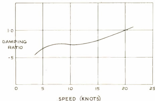
FIG. 7. Typical variation of damping ratio with submarine speed.
