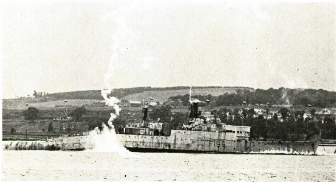
H.M.S. "Roebuck" and H.M.S. "Broadsword" are being used by the Naval Construction Research Establishment for trials this summer as part of an investigation on the effectiveness of underwater explosions. The photograph shows the "Roebuck" at the instant of maximum "jack-knifing" abreast the charge (approximately 8^{\circ} ). The ships have been extensively instrumented to measure displacement, velocity, acceleration and strain and are beached after each test to inspect the structural damage. The tests form part of a U.S./U.K. co-operative programme of explosive research, the Americans having already conducted tests against two of the ships earlier this year.
