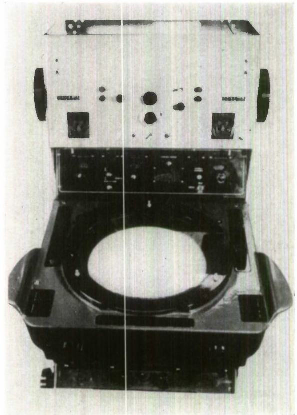
FIG. 7. The Decca "Alpine" precision ranging unit.
