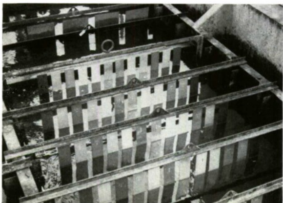
FIG. 11. Frames in position on one of the rafts.
