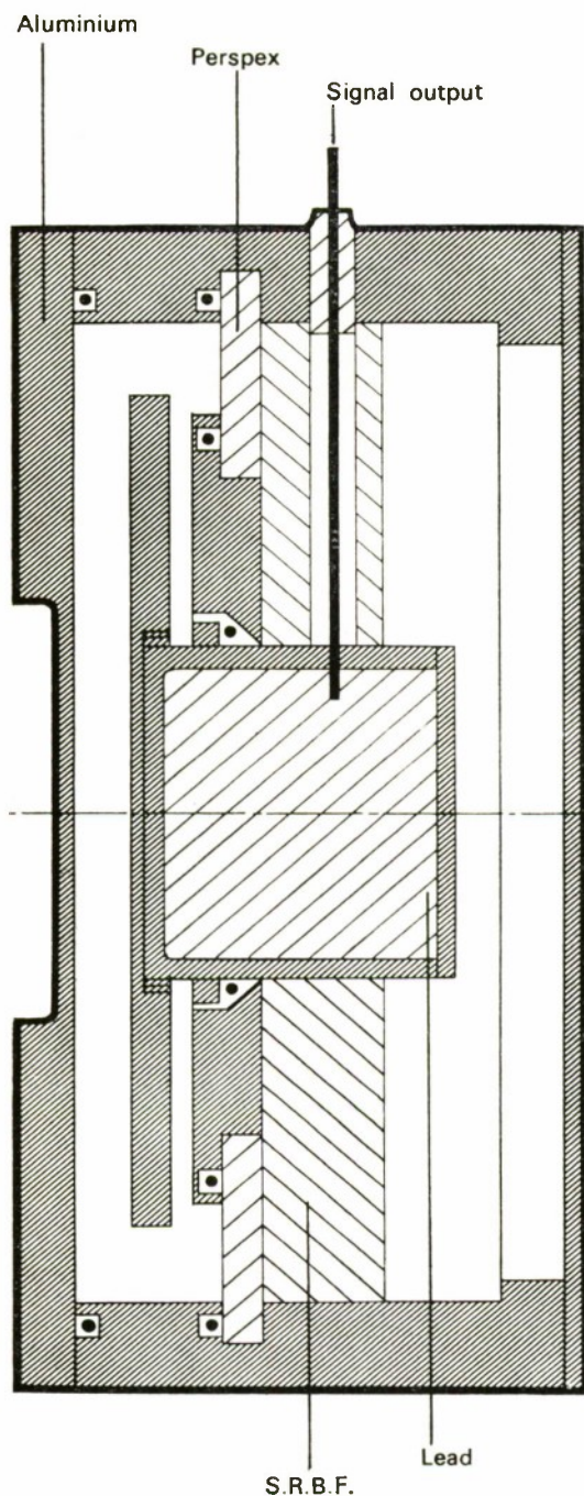
FIG. 1. Sectional side elevation of Pill-Box.
