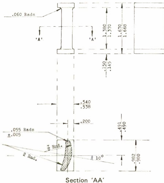
FIG. 7. Test specimen
