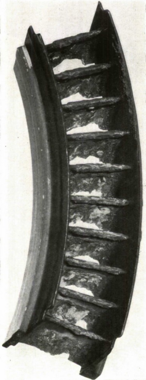
FIG. 1. Corroded nozzle segment from engine test at 0.5 to 1.0 ppm salt
