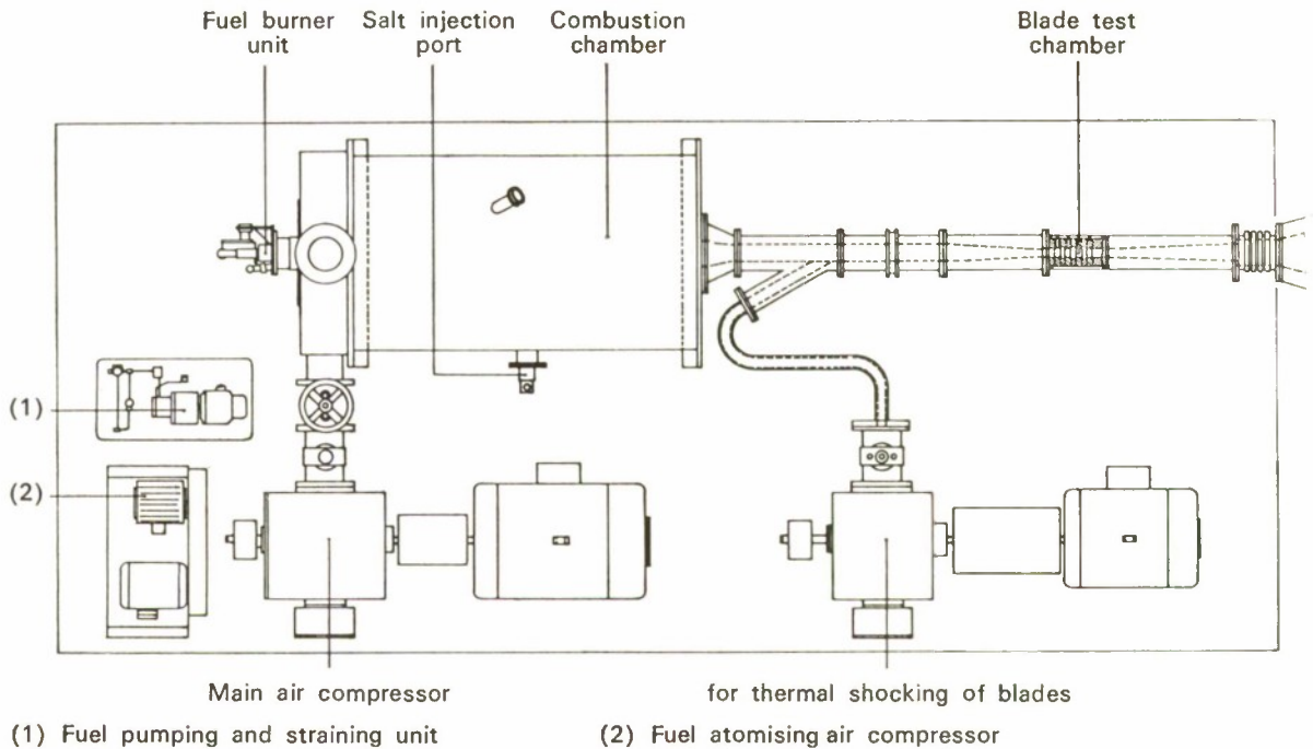
FIG. 6. A.M.L. corrosion test rig
