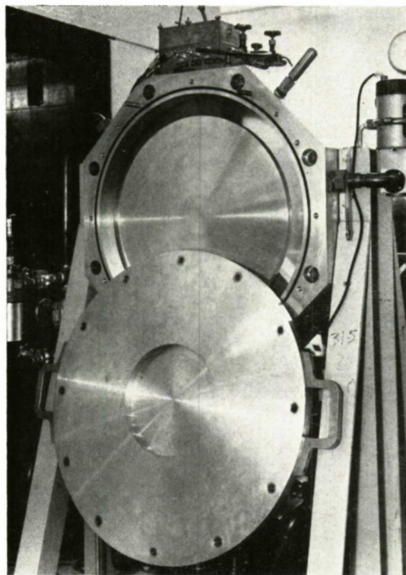
FIG. 2. Pill-Box with front plate removed.
