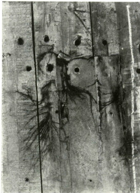
FIG. 1. Mahogany planking from hull of coastal minesweeper decayed by Coniophora cerebella
