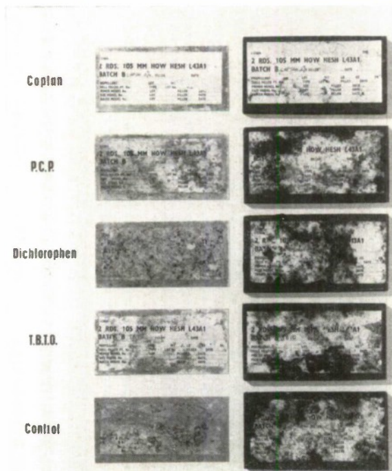
FIG. 2. Relative efficiency of fungicide-containing label adhesives as shown by exposure to four weeks soil burial test.
