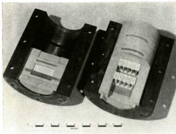
FIG. 9. Specimens and test chamber
