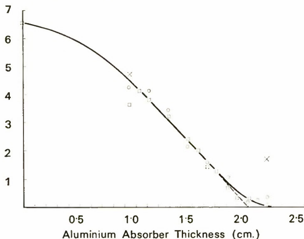
FIG. 5. Electron beam energy. Plot of Pill-Box current on arbitrary scale against thickness of aluminium alloy absorber in centimetres. Intercept of dotted line on axis gives the extrapolated range. Points enclosed by circles were made at a pressure between 29 and 45 mtorr, those by squares at atmospheric pressure and those indicated by crosses at higher beam energy and lower beam current.
