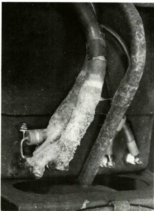
FIG. 3. Mould growth on P.V.C. cable insulation of radio equipment.
