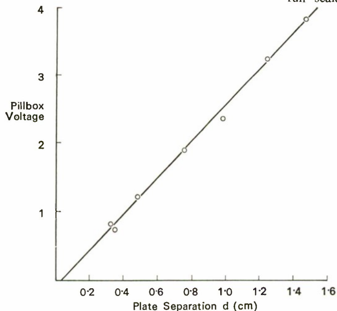
FIG. 3. Pill-Box voltage as a function of separation between the plates. Voltage on an arbitrary scale, plate separation in centimetres.
