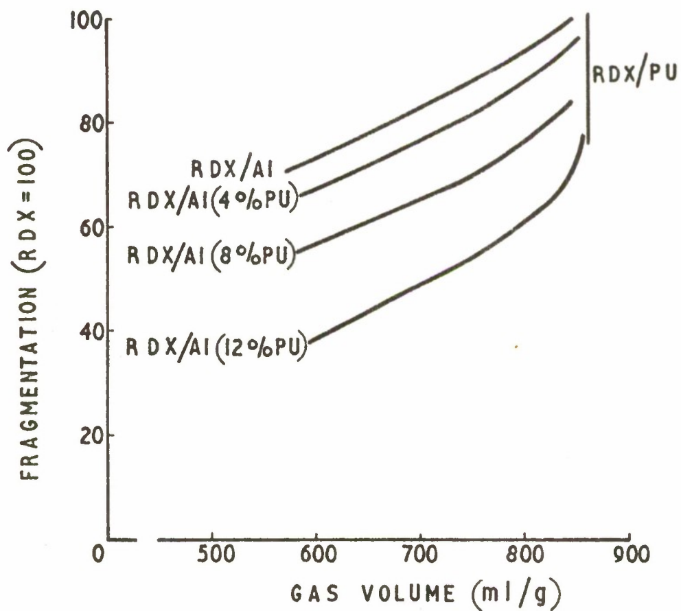
FIG. 6 VOLUME OF GAS PRODUCED AND FRAGMENTATION
