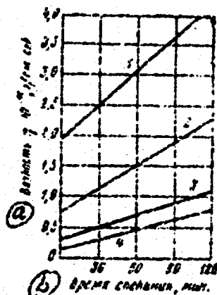
Fig 6. Shearing viscosity of compacted chromium carbide vs time of sintering at temperatures of: 1 - 1370^\circ , 2 - 1480^\circ , 3 - 1540^\circ , 4 - 1590^\circ (a) viscosity 10^{-11} , g/cm-sec (b) sintering time, min
