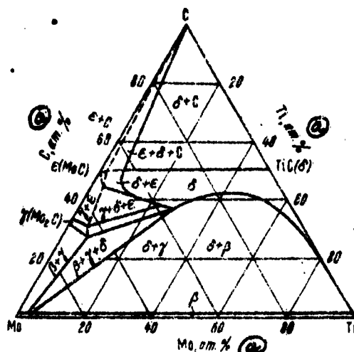
Fig 5. Isothermal section of ternary system Ti-C-Mo (Ref 2)
