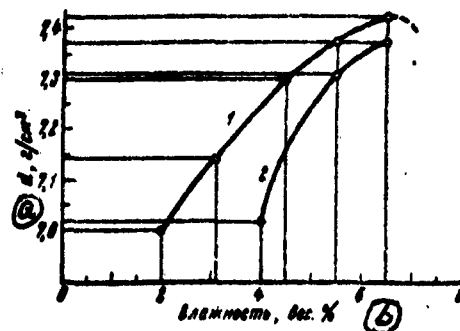
Fig 5. Density of compacts of a mixture of tungsten carbide and 20% Co powders as a function of the moisture content of the powders for vibration pressing:
