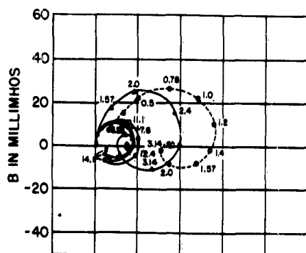
FIG. 7(e) MEASURED ADMITTANCE IN THE SOLUTION WITH \epsilon_r = 78 , \frac{\sigma}{\omega\epsilon_r\epsilon_0} = 0.53
