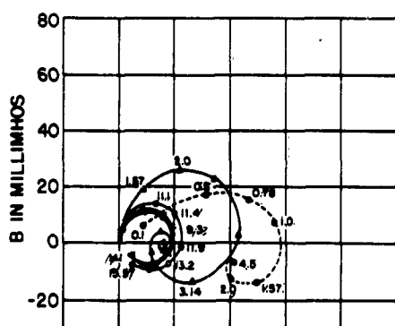
FIG. 7(f) MEASURED ADMITTANCE IN THE SOLUTION WITH \epsilon_r = 77 , \frac{\sigma}{\omega\epsilon_r\epsilon_0} = 1.06
