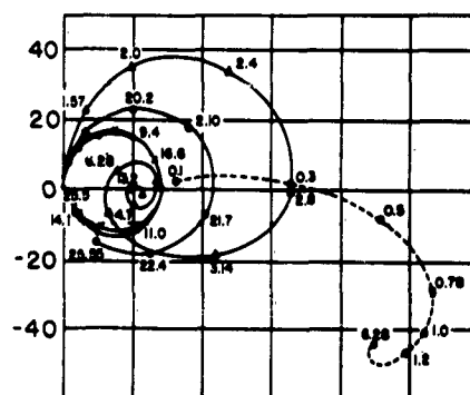
FIG. 7(i) MEASURED ADMITTANCE IN THE SOLUTION WITH \epsilon_r = 70 , \frac{\sigma}{\omega\epsilon_r\epsilon_0} = 6.2
