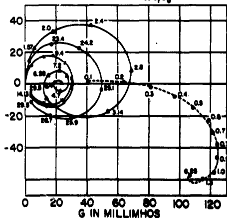
FIG. 7(j) MEASURED ADMITTANCE IN THE SOLUTION WITH \epsilon_r = 69 , \frac{\sigma}{\omega\epsilon_r\epsilon_0} = 8.8
