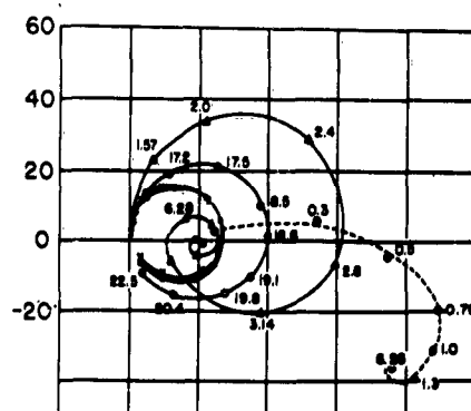
FIG. 7(h) MEASURED ADMITTANCE IN THE SOLUTION WITH \epsilon_r = 72 , \frac{\sigma}{\omega\epsilon_r\epsilon_0} = 4.4
