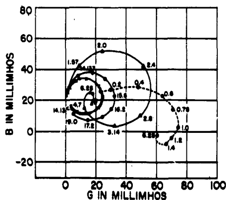
FIG. 7(g) MEASURED ADMITTANCE IN THE SOLUTION WITH \epsilon_r = 74 , \frac{\sigma}{\omega\epsilon_r\epsilon_0} = 2.64
