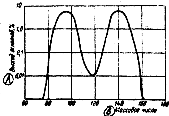
Figure 3. Yield of various fission fragments of uranium-235 upon its irradiation with thermal neutrons. A = Fragment yield, %; B = Mass number.
