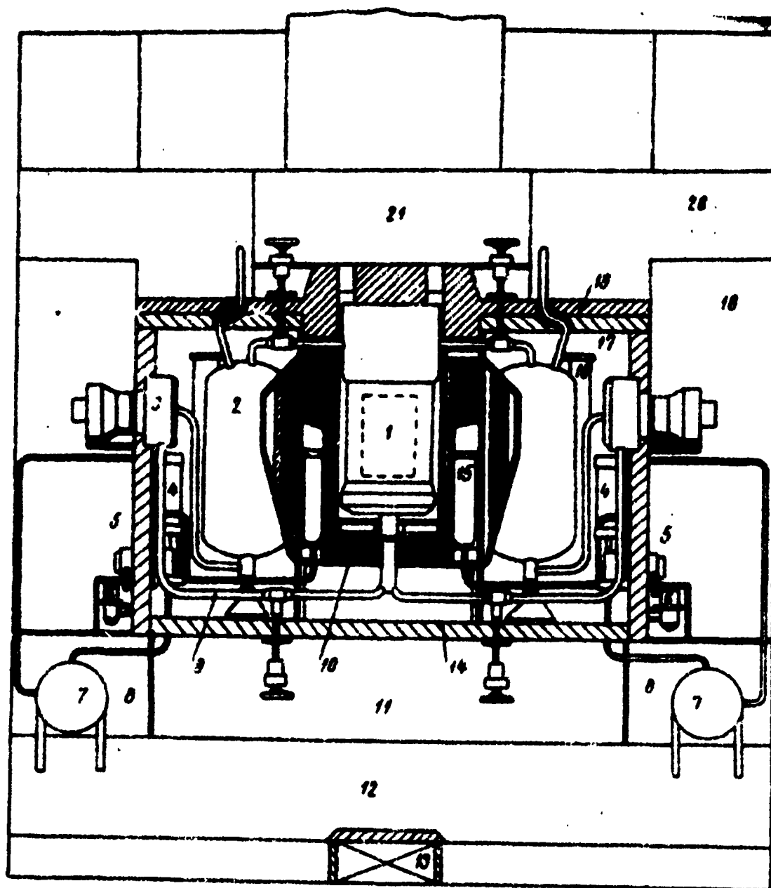
Figure 14. Cross-sectional view of central subcore of the atomic icebreaker "Lenin". [See legend next page].
