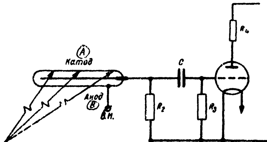
Figure 24. Diagram of gas-discharge counter. A = Cathode; B = Anode.
