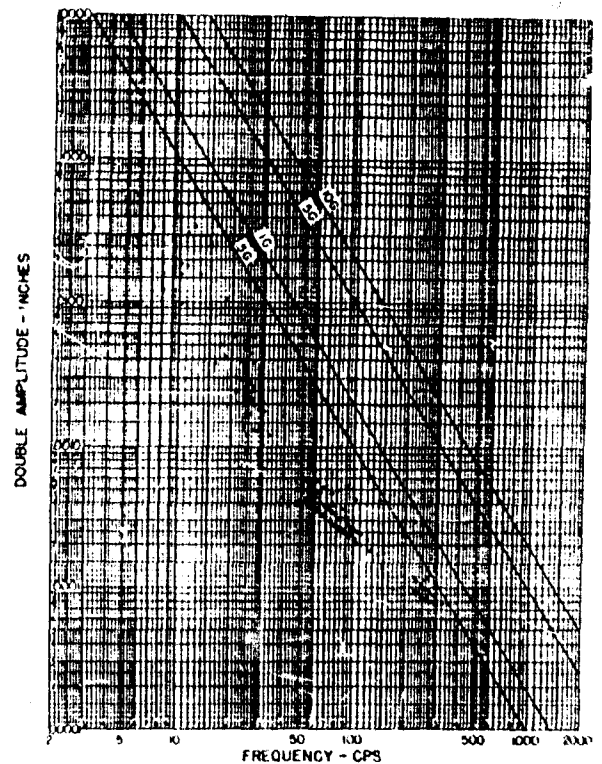
Figure 44. DIRECTION VERT LOCATION SHOCKMOUNTED EQUIPMENT BACK IN FUSE SECTION F 3 185
