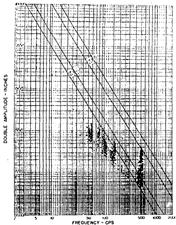
Figure 53. DIRECTION LAT LOCATION FWD END OF ACCESSORY SECTION OF J-57-P15 ENGINE F5 56B
