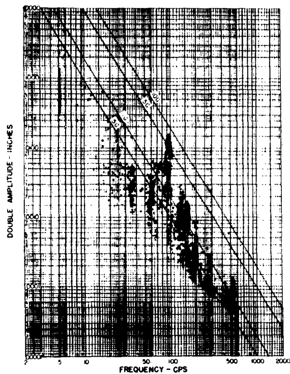
Figure 28. DIRECTION: VERT. LAT. B F/A LOCATION: BRUSH BAND OF 400A DC GEN
