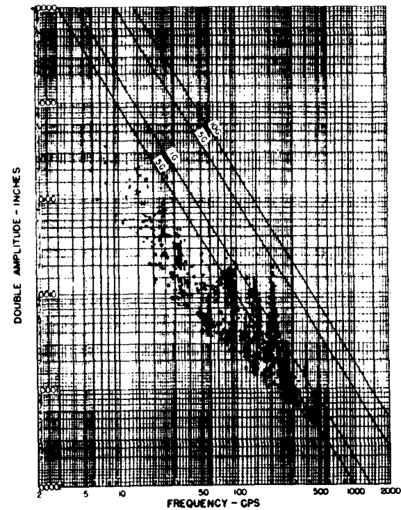
Figure 30. DIRECTION: VERT. LAT. B F/A LOCATION: FORWARD END OF FORWARD COMPRESSION SECTION
