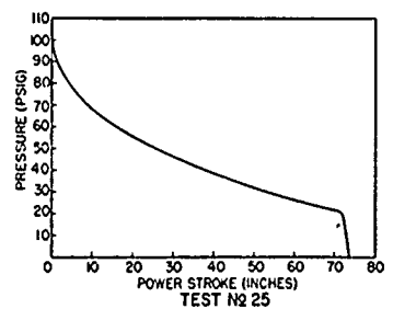
FIG 20 INTERNAL BLAST PRESSURE - POWER STROKE PLOTS FOR TESTS No 2, 29, 35, 23, 25, AND 24
